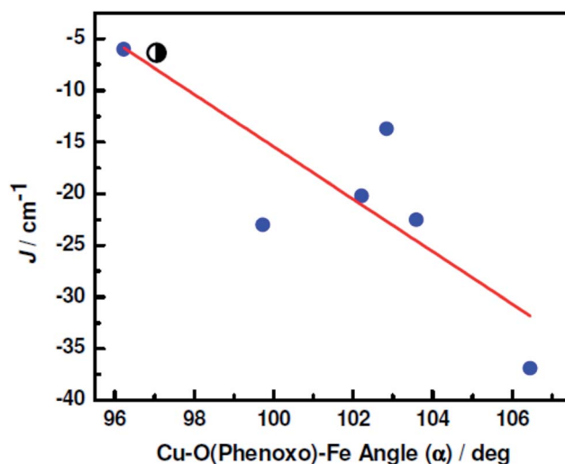
Fig. 11 J versus \text{Cu}\text{--O}(\text{phenoxo})\text{--Fe} bridge angle magneto-structural correlation in diphenoxo-bridged \text{Cu}^{\text{II}}\text{Fe}^{\text{II}} compounds. Blue filled circles: data of previous compounds. Black-white half-filled circle: data of compound 4 .
