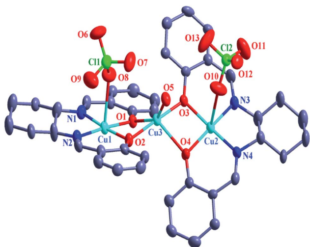
Fig. 1 ORTEP drawing (ellipsoid probability at 30%) of the structure of [\{\text{Cu}^{\text{II}}\text{L}(\text{ClO}_4)\}_2\text{Cu}^{\text{II}}(\text{H}_2\text{O})] \cdot 2\text{H}_2\text{O} (1). All hydrogen atoms are omitted for clarity.
