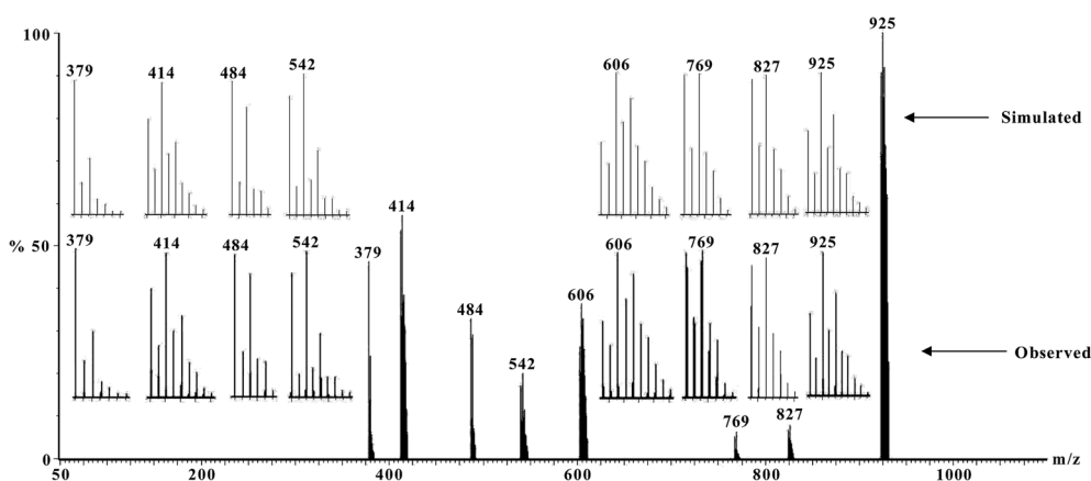
Fig. 5 Electrospray ionization mass spectrum in positive mode (ESI-MS positive) of [(\text{Cu}^{\text{II}}\text{L}(\text{ClO}_4))\{\text{Ni}^{\text{II}}(\text{H}_2\text{O})_2\}\{\text{Cu}^{\text{II}}\text{L}\}]\text{ClO}_4 \cdot \text{CH}_3\text{COCH}_3 ( 2 ) in acetonitrile, showing observed and simulated isotopic distribution patterns.
