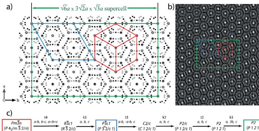
Fig. 6 (a) Projection of the Cs_8Zn_{18}Sb_{28} clathrate superstructure, with the Pm\bar{3}n subcell (red), the P\bar{3}c1 supercell (blue), and P2 supercell (green) emphasized. Note the projection of the subcell is along the [111]_C direction. (b) [001] HAADF-STEM image of Cs_8Zn_{18}Sb_{28} with model unit cells drawn over: P2 (green), P\bar{3}c1 (blue), and Pm\bar{3}n (red). (c) Diagram showing the group-subgroup relationship between the ideal type-I clathrate Pm\bar{3}n subcell and the P2 supercell.
