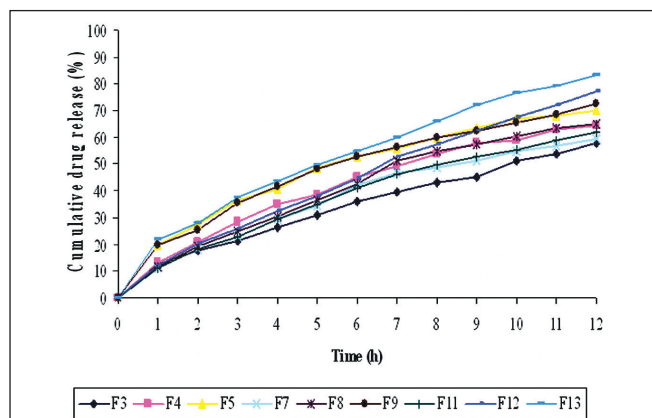
Figure 2: Comparison of in vitro release profiles of HPMC matrix tablets of diltiazem hydrochloride
