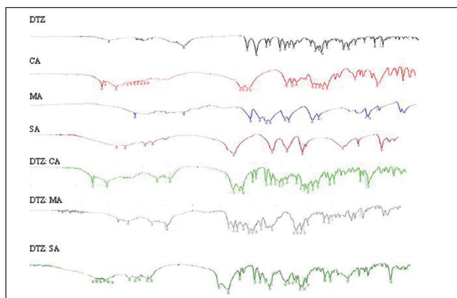
Figure 1: FT-IR spectra of diltiazem (DTZ) HCL, citric acid (CA), malic acid (MA), succinic acid (SA), and physical mixture of DTZ with CA, MA, and SA, respectively
