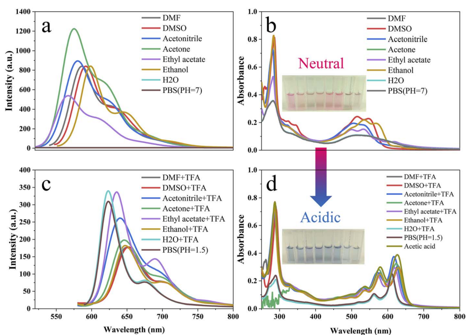
Fig. 4 Fluorescence (a) and UV-vis (b) spectra of the R-CDs (10 μg mL -1 ) in different solvents under neutral conditions. \lambda_{\text{ex}} = 534 nm. Fluorescence (c) and UV-vis (d) spectra of the R-CDs in different solvents under acidic conditions (concentration of TFA added: 2.7 \times 10^{-4} mol L -1 ). \lambda_{\text{ex}} = 570 nm.
