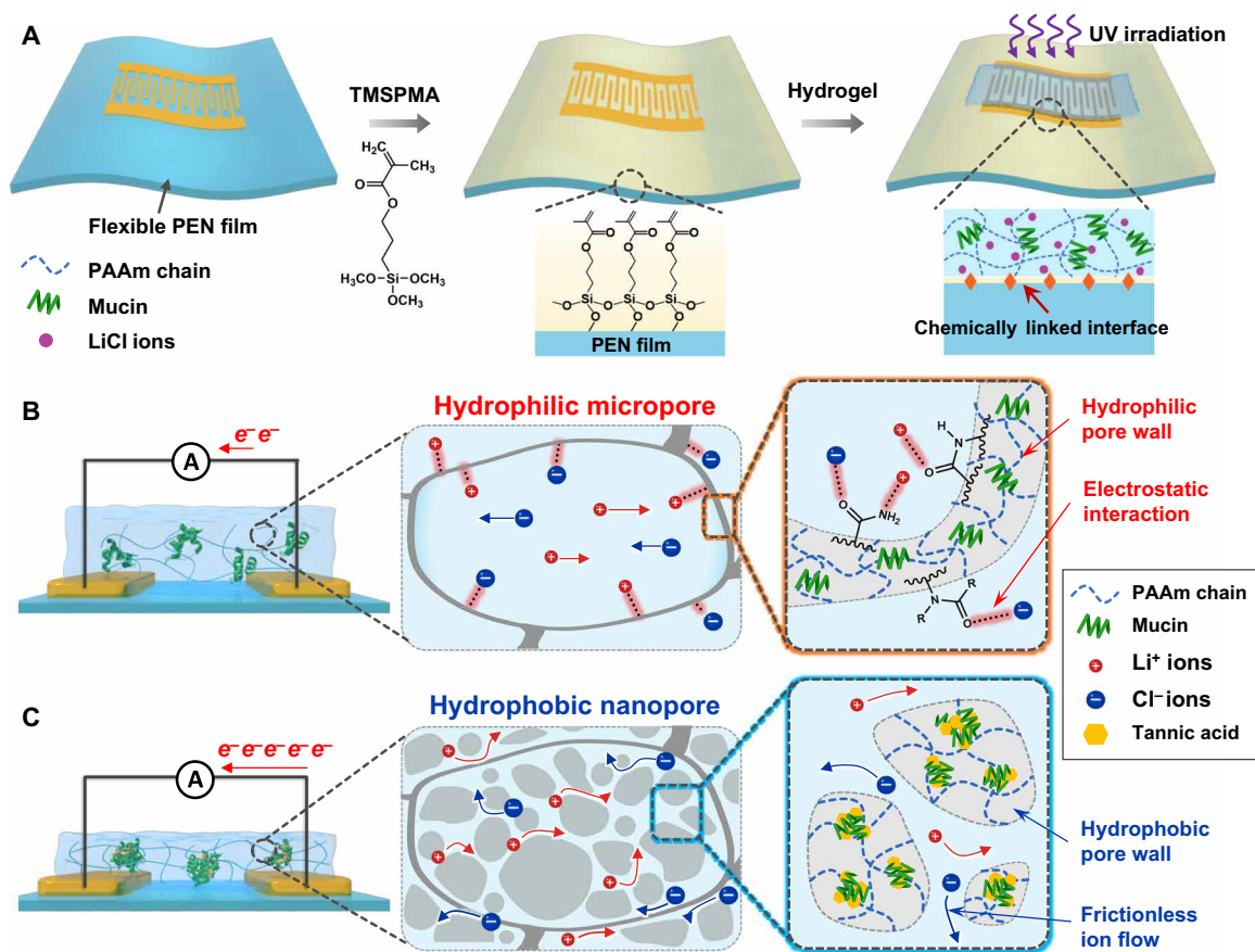
Fig. 3. Design of the flexible artificial tongue. (A) The fabrication process of the flexible astringency sensor. (B) Schematic illustration of the working principle of the astringency sensor before TA treatment (left); a hydrophilic micropore in the hydrogel (center); magnified pore walls visualizing the electrostatic interaction–limited ion flow (right). (C) Schematic illustration of the working principle of astringency sensor after TA treatment (left); a hierarchical micro/nanopore in the hydrogel (center); magnified pore walls of hydrophobic nanopore visualizing enhanced ion flow (right).
