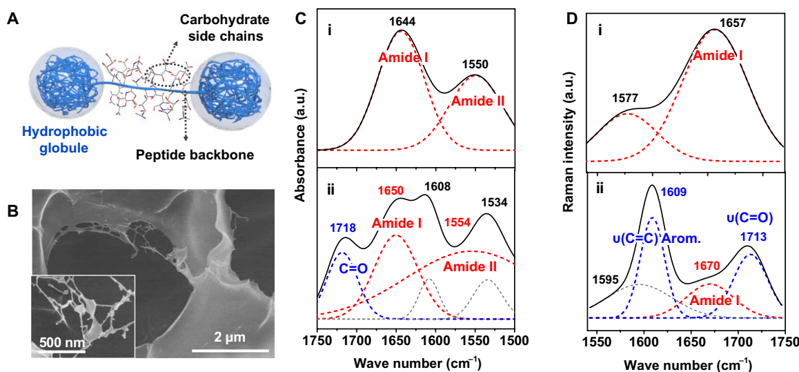
Fig. 2. Binding mechanism of mucin and TA. (A) Schematic illustration of mucin. (B) SEM image of the mucin polymer dispersed in the PAAm hydrogel network; inset image is magnified part of the pore edge. (C) FTIR spectra of (i) mucin and (ii) mixture of mucin and TA. (D) Raman spectra of (i) mucin and (ii) mixture of mucin and TA. a.u., arbitrary unit.
