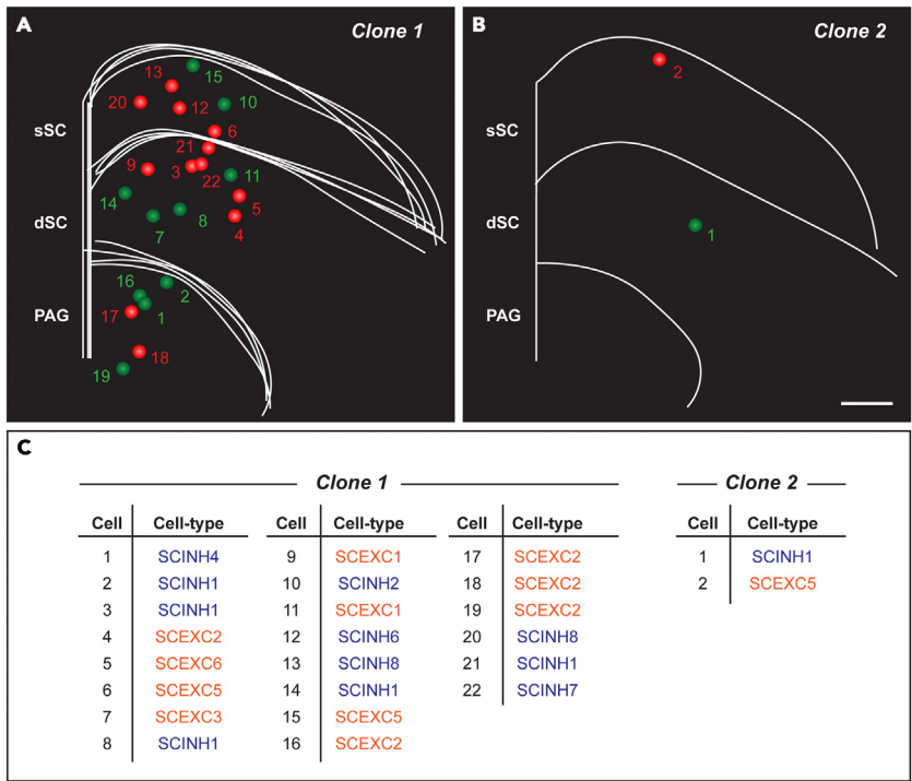
Figure 5. Representative MADM clones with mapped cell-type identity of individual cells (A and B) Reconstructed illustrations of 2 MADM clones in the SC are shown. Red and green spheres represent the positions of individual sampled MADM-labeled cells. Layers are separated by lines and marked as superficial superior colliculus (sSC), deep superior colliculus (dSC) and periaqueductal gray (PAG). A Z-projection from 4 acute slices are shown for Clone 1 which was induced at E10.5 and contains 22 neurons (A). Clone 2 was induced at E12.5 and contains 2 neurons in a single slice (B). (C) Cell-type identity of individual cells is listed for both clones. Inhibitory types are written in blue while excitatory types are in orange. Cell types are annotated based on published dataset 19 and renamed in our original publication. 1 Scale bars = 200 \mu m in (A–B).
