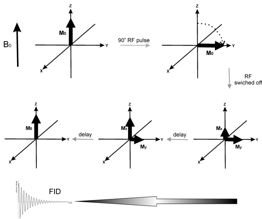
Figure 4. The scheme presenting the main idea of MRI. Upper part: The variable B_1 field in the form of a radiofrequency (RF) pulse rotates the magnetization to the transverse plane. Lower part: After the RF pulse is switched off, the system relaxes in time until equilibrium is reached, generating a FID signal. The processes leading to thermal equilibrium after RF pulse can be described as longitudinal (spin-lattice) relaxation, with characteristic constant T_1 , and transverse (spin-spin) relaxation characterized by T_2 . The first process occurs due to the dissipation of the absorbed energy to the surrounding environment, while the second results from the energy redistribution among the nuclei. The MRI contrasts improve the quality of the MRI image via influencing T_1 or T_2 of the surrounding tissue. Water protons in different tissues have different T_1 and T_2 , a phenomenon that provides MRI contrast. T_1 is shortened by the interactions of the observed nuclei with paramagnetic agents and by a limited mobility of H_2O molecules (observed in more viscous tissues). T_2 is also shortened by lower molecular mobility. SPIONs are mainly negative T_2 contrast agents. When accumulated in the tissue, they shorten T_2 , decreasing signal intensity, and provide a negative contrast enhancement. It is also suggested that if SPIONs' particles are small enough (<10 nm), they could act as T_1 positive contrast agents [40].
