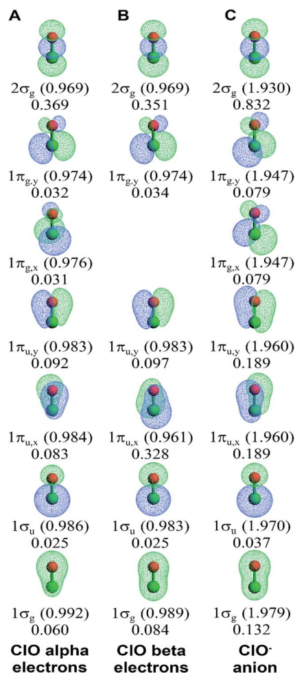
Fig. 7 Bond order component analysis (BOCA) for the ClO (doublet) molecule and ClO - (singlet) anion using the natural spin-orbitals. Orbital occupancies are given in parentheses. Bond order components are listed without parentheses. The oxygen atom is displayed in red, while the chlorine atom is displayed in green.
