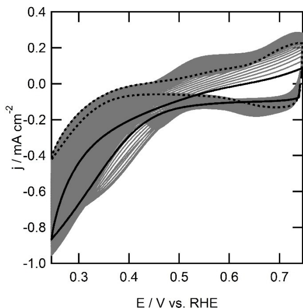
Figure 9. Electrochemical behavior of a gold electrode ( 0.05 \text{ cm}^2 geometric surface area) grafted with 1 in presence of oxygen in 0.1 \text{ M} phosphate buffer with 0.05 \text{ M} NaCl acidified to pH 4 with HCl at 100 \text{ mV s}^{-1} . First scan is depicted in black, 200 th scan is depicted in dotted black line.
