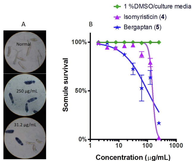
Figure 3. Effect of isomyristicin and bergapten on the survival of S. mansoni schistosomula. (A) Trypan blue stained images (20 \times ) showing 100% lethality to schistosomula (250 \mu\text{g/mL} compound concentrations) and first signs of lethal effects observed at 31.2 \mu\text{g/mL} of the two compounds tested. Deep blue staining signifies a dead parasite. (B) The effect of the two compounds on schistosomula survival at different concentrations (250–1.95 \mu\text{g/mL} ). The data was generated from triplicate samples obtained from two independent studies.
