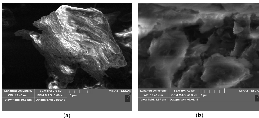
Figure 2. SEM of \beta -CD(AN-co-AA) hydrogel particles in different resolution size 10 \mu\text{m} (a) and 1 \mu\text{m} (b).
