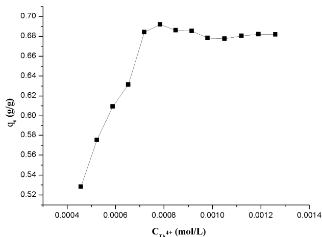
Figure 9. Effect of the initial concentration of \text{Th}^{4+} on the adsorption behavior onto \beta -CD(AN-co-AA).
