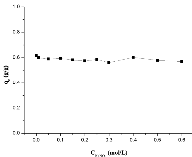
Figure 7. Effect of the ionic strength of the solution on the adsorption of Th(IV) onto \beta -CD(AN-co-AA).
