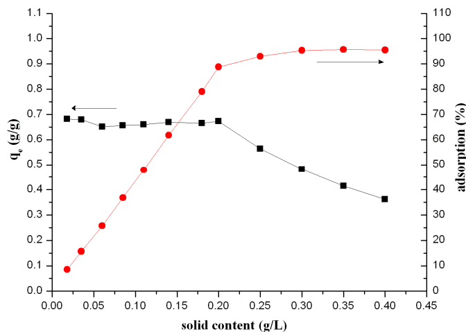
Figure 8. Effect of solid content on the adsorption of Th(IV) onto \beta -CD(AN-co-AA), square point show the value of q_e (g/g) and dot show the value of “adsorption %”.
