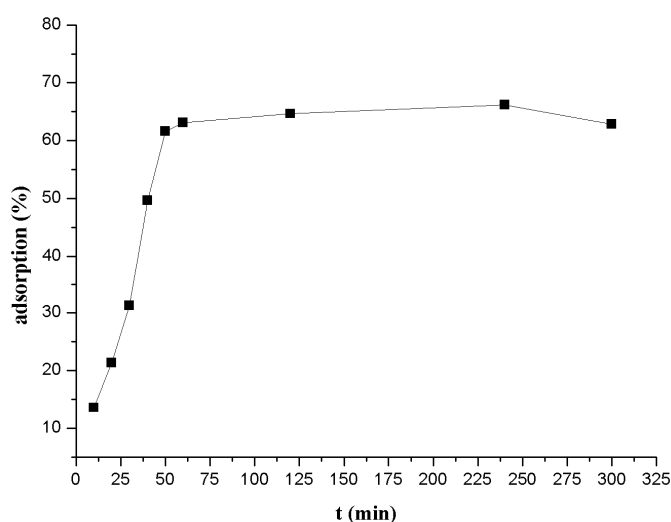
Figure 4. Effect of equilibrium time on Th(IV) adsorption onto \beta -CD(AN-co-AA).
