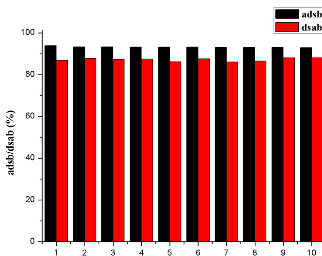
Figure 12. The amount of Th 4+ adsorbed as a function of the adsorption-desorption cycle. Adsorption (adsb) and desorption (dsab) cycles: adsorption-sample volume = 5.0 mL, Th(IV) concentration = 6.5334 \times 10^{-4} mol/L, adsorption dose ( \beta -CD(AN-co-AA)) = 0.30 g/L, initial pH = 2.95 \pm 0.05 , equilibration time = 4 h; desorption-sample volume = 5.0 mL of 0.09 M HNO 3 .
