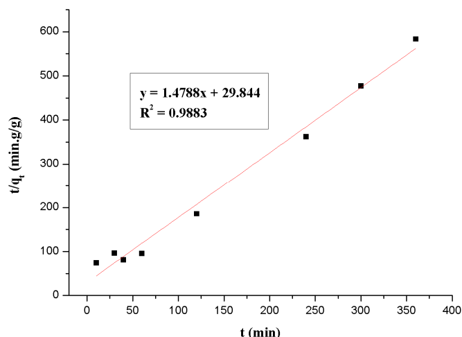
Figure 5. Test of pseudo-second-order adsorption kinetics plot for Th(IV).
