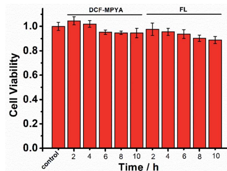
Fig. 7 Biological toxicity of MCF-7 cells in the presence of DCF-MPYA (20 μM), and FL (20 μM) was determined after different incubation time. Mean values and standard deviations are obtained from three independent experimental determinations.
