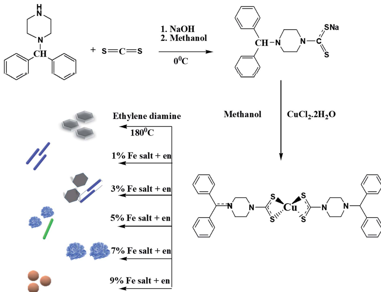
Scheme 1 Synthesis of single source precursor, \text{CuS}/\text{Cu}_2\text{S} and Fe-doped \text{CuS}/\text{Cu}_2\text{S} .
