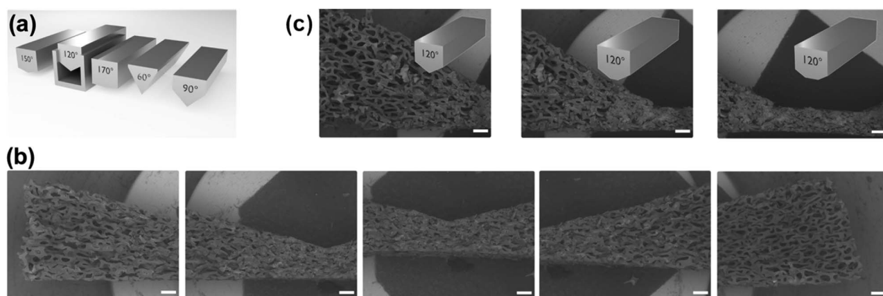
Fig. 3 (a) Schematic deformation procedure leading to a bidirectional structural gradient organosilica material. SEM micrographs (scalebars = 500 \mu\text{m} ) of a bidirectional 150° gradient (b) and variation of the extension of the pore-small region of a 120° bidirectional gradient (c).
