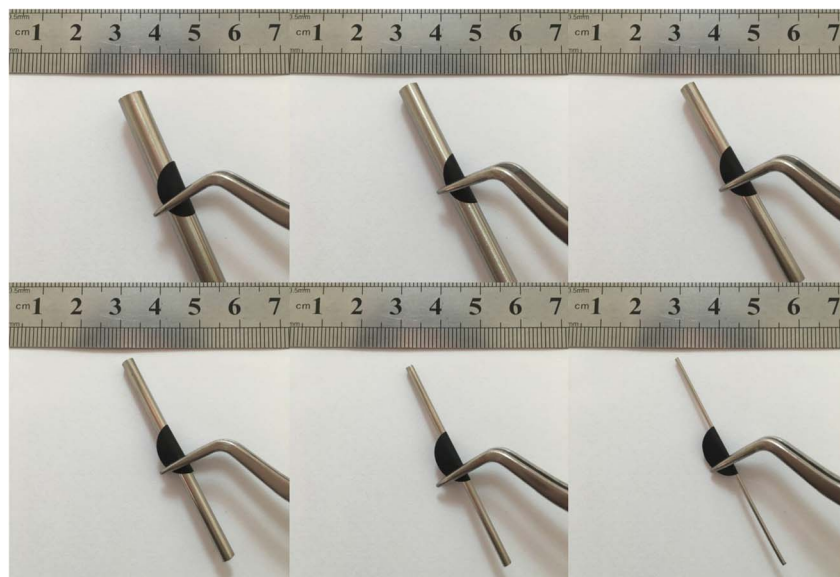
Fig. 5 A set of digital images of the curly S/CNT/G films bent around rods.
