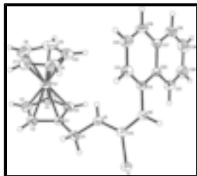
Fig. 1. The molecular structure of the title compound, showing the atomic numbering and 30% probability displacement ellipsoids.
