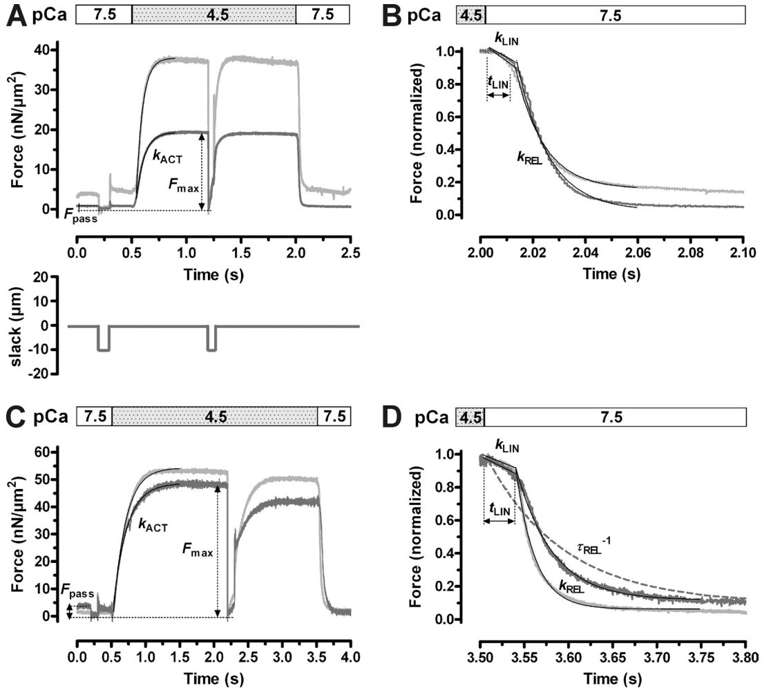
Figure 3. Representative force transients obtained at 10°C from isometrically mounted (as shown in Fig. 1, E and O) skeletal (A and B) and cardiac (C and D) myofibrils. (A) A full contraction–relaxation cycle of a skeletal myofibril isolated from skinned myotomes of zebrafish larvae (light gray trace; k_{\text{ACT}} = 20 \text{ s}^{-1} , F_{\text{max}} = 38 \text{ nN}/\mu\text{m}^2 , and F_{\text{pass}} = 3.4 \text{ nN}/\mu\text{m}^2 ; see Video 1 ) and adult zebrafish (dark gray trace; k_{\text{ACT}} = 13 \text{ s}^{-1} , F_{\text{max}} = 20 \text{ nN}/\mu\text{m}^2 , and F_{\text{pass}} = 1.2 \text{ nN}/\mu\text{m}^2 ; see Video 2 ). Ca 2+ concentration is rapidly (10 ms) changed from pCa 7.5 to 4.5 and back to 7.5 to induce contraction and the relaxation, respectively. Before Ca 2+ activation, the passive force ( F_{\text{pass}} ) and, during Ca 2+ activation, the maximum generated force ( F_{\text{max}} ) are determined, respectively, by transiently slackening–restretching the initially pre-stretched myofibrils at SL = 1.15 \times SL_0 . (B) Recordings on an expanded time scale of the biphasic normalized force decay shown in A for larvae (light gray trace; k_{\text{LIN}} = 10.3 \text{ s}^{-1} , t_{\text{LIN}} = 12 \text{ ms} , and k_{\text{REL}} = 98 \text{ s}^{-1} ) and for adult zebrafish (dark gray trace; k_{\text{LIN}} = 7.6 \text{ s}^{-1} , t_{\text{LIN}} = 14 \text{ ms} , and k_{\text{REL}} = 79 \text{ s}^{-1} ). (C) A full contraction–relaxation cycle of a cardiac myofibril isolated from the myocardium of adult zebrafish (dark gray trace; k_{\text{ACT}} = 5.2 \text{ s}^{-1} , F_{\text{max}} = 47 \text{ nN}/\mu\text{m}^2 and F_{\text{pass}} = 3.3 \text{ nN}/\mu\text{m}^2 ; see Video 3 ) and from murine papillary muscles (light gray trace; k_{\text{ACT}} = 5.8 \text{ s}^{-1} , F_{\text{max}} = 52 \text{ nN}/\mu\text{m}^2 , and F_{\text{pass}} = 1.8 \text{ nN}/\mu\text{m}^2 ; see Video 4 ) subjected to a protocol similar to that described for A. (D) Normalized force transients of the biphasic relaxation shown on an expanded time scale for a cardiac myofibril in C: zebrafish (dark gray trace; k_{\text{LIN}} = 2.3 \text{ s}^{-1} , t_{\text{LIN}} = 46 \text{ ms} , k_{\text{REL}} = 25 \text{ s}^{-1} ) and mouse (light gray trace; k_{\text{LIN}} = 2.1 \text{ s}^{-1} , t_{\text{LIN}} = 32 \text{ ms} , and k_{\text{REL}} = 42 \text{ s}^{-1} ). Dashed curve (shown only for the zebrafish cardiac myofibril) is the simulated force decay with the rate constant 1/\tau_{\text{REL}} calculated from kinetic parameters of the force relaxation using Eq. 1 ( \tau_{\text{REL}}^{-1} = 12.3 \text{ s}^{-1} for a zebrafish cardiac myofibril; for comparison, \tau_{\text{REL}}^{-1} = 18.5 \text{ s}^{-1} for a murine cardiac myofibril). Mono-exponential increase (myofibril contraction) and biphasic decay comprised of a linear followed by a mono-exponential phase of decay functions were used to fit (thin black lines) force transients, yielding the kinetic parameters. Steady-state and kinetic force parameters ( F_{\text{pass}} , F_{\text{max}} , k_{\text{ACT}} , k_{\text{LIN}} , t_{\text{LIN}} , k_{\text{REL}} , and \tau_{\text{REL}}^{-1} ) are shown only for skeletal and cardiac myofibrils of the adult zebrafish.
