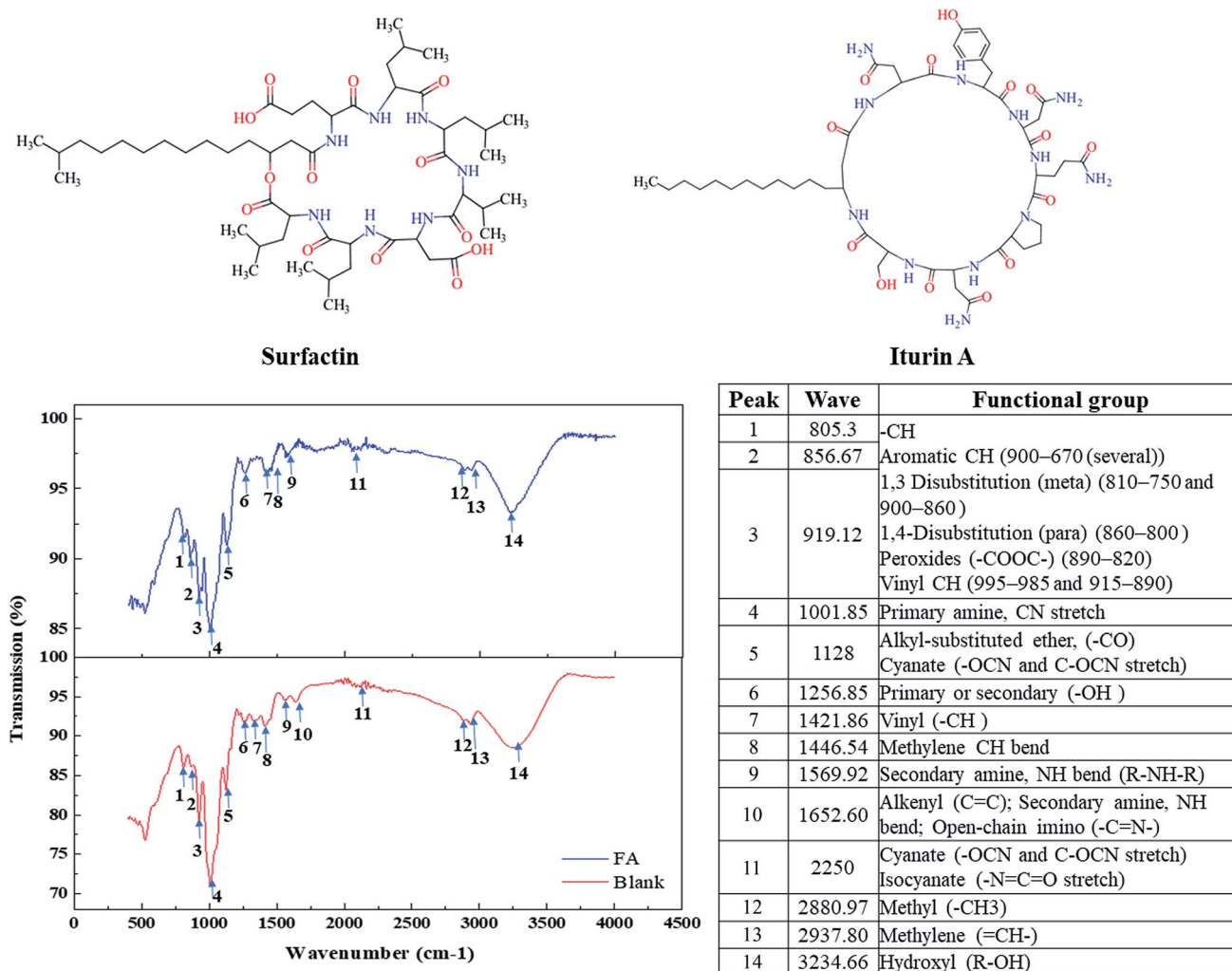
Fig. 3 FTIR analysis of biosurfactant produced by Bacillus strains with FA-based platform.
