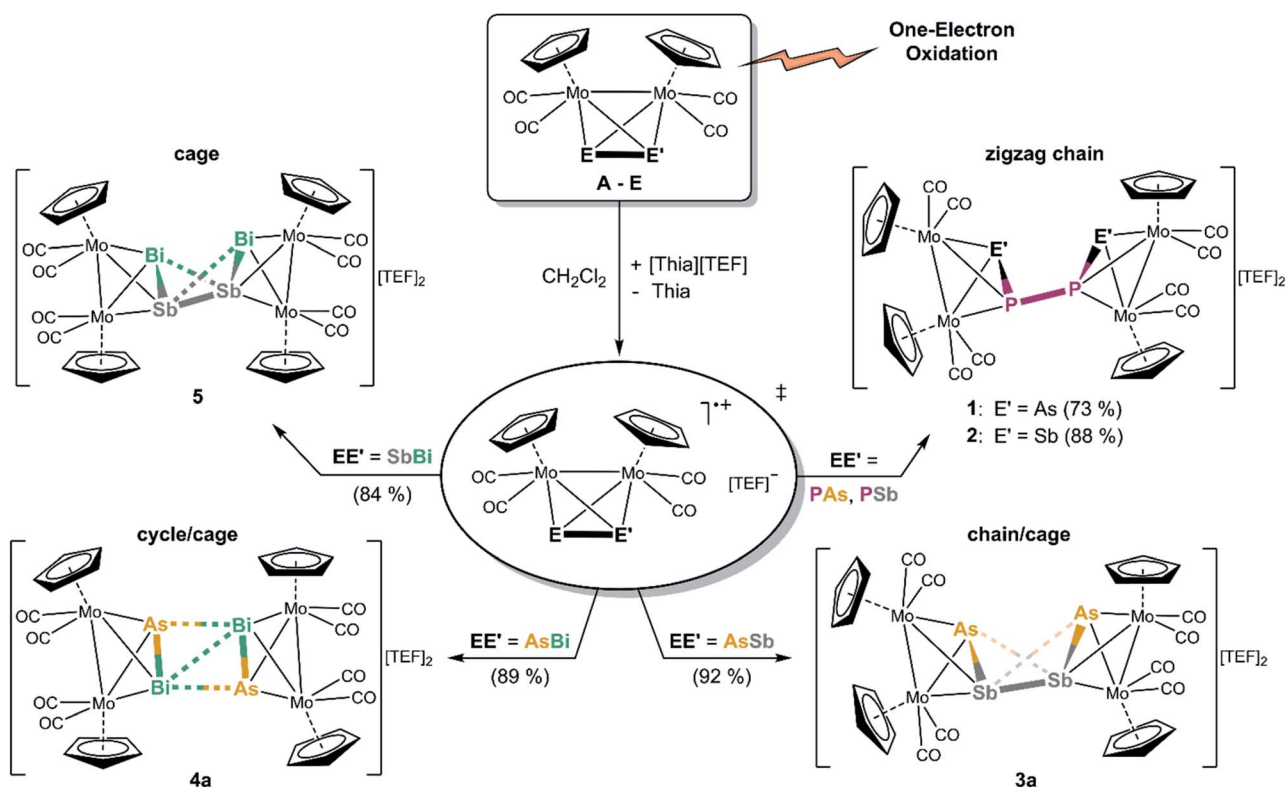
Scheme 2 Oxidation of the tetrahedral hetero-dipnictogen complexes [{CpMo(CO) 2 } 2 (μ,η 2 :η 2 -EE')] (EE' = PAs (A), PSb (B), AsSb (C), AsBi (D), SbBi (E)) resulting in dimerization reactions leading to dicationic E 2 E' 2 chains, cages and cycles. Isolated yields are given in parentheses.
