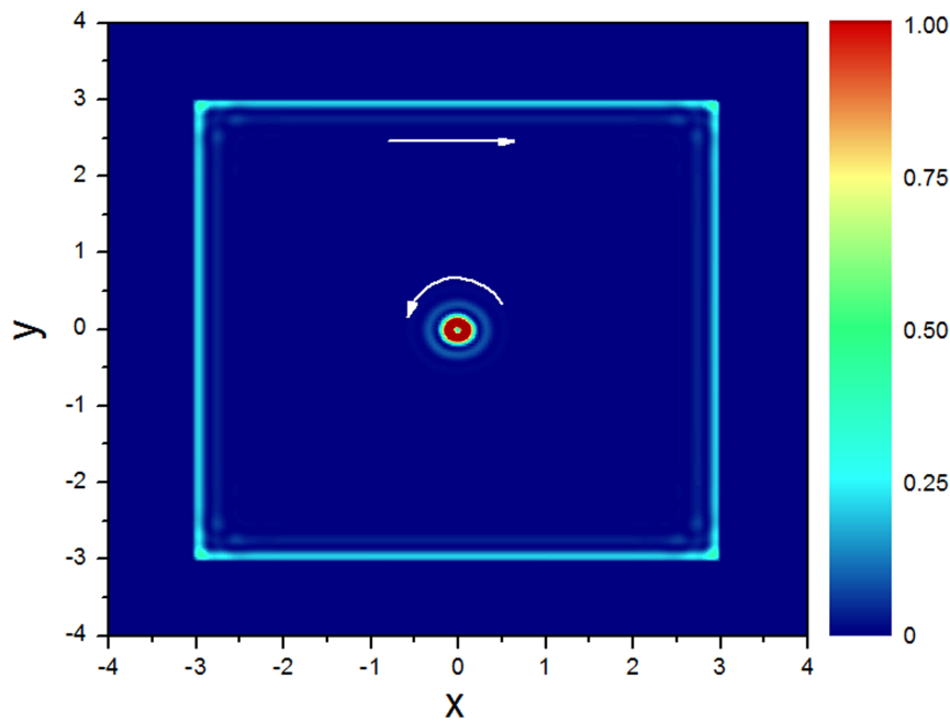
Figure 3 | Manifestation of photonic zero-energy modes at a vortex and at edges. The mode at the vortex propagates counter-clockwise around the center vortex core, while the mode at the edge propagates clockwise. Azimuth-dependent off-diagonal elements in permittivity and permeability tensors are introduced to mimic a vortex with a singularity at the center.
