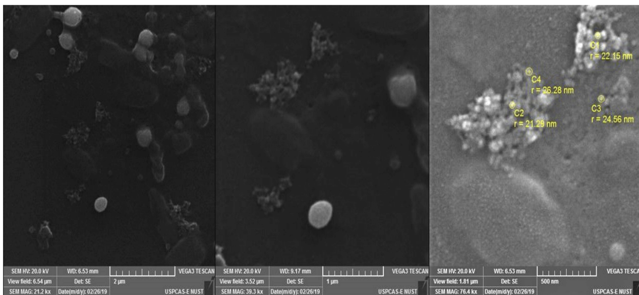
Figure 5 Scanning electron microscopic images of selenium nanoparticles derived from Foeniculum vulgare Mill. seed extract at 2 μm, 1 μm and 500 nm depicting spherical to irregular morphology of selenium nanoparticles.
