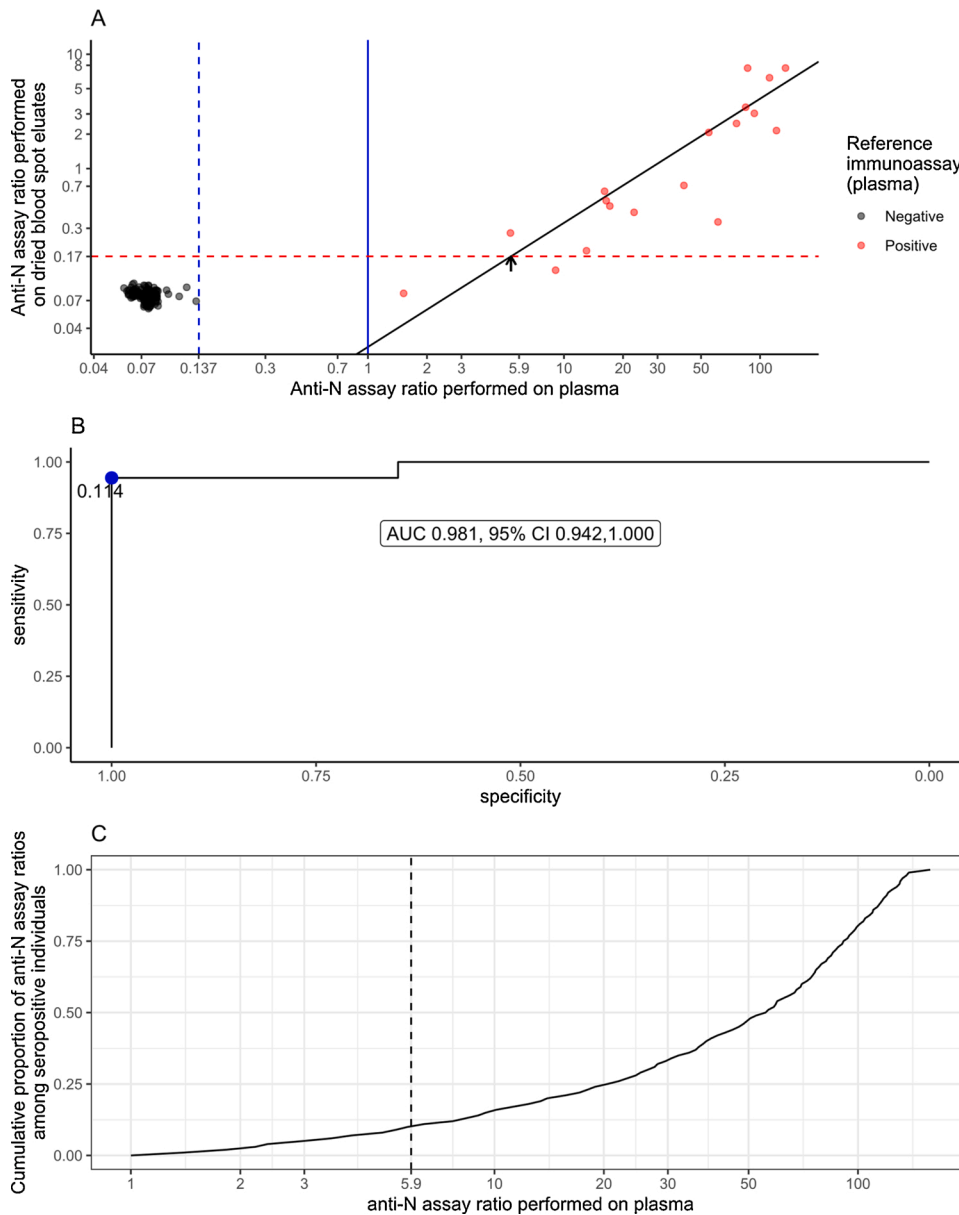
Fig. 4. Immunoassay signals from plasma and DBS samples. Figure 4 (A) The relationship between antibody ratios obtained using Roche Elecsys immunoassays for plasma (reference test, x-axis) vs. paired dried blood spots (index test, y-axis). Samples positive in the plasma immunoassay are in red. Solid blue line: manufacturer’s cutoff for plasma samples (1). Red dotted line: experimental cutoff ten median absolute deviations above the reference test negative median for DBS (index test) samples (n = 177). Blue dotted line: experimental cutoff ten median absolute deviations above the reference test negative median for plasma (reference test) samples. Solid black line: regression of index test immunoassay ratios on reference test immunoassay ratios. Arrow: estimate of limit of detection. (B) Receiver operator curve, showing sensitivity/specificity of DBS usage, relative to an immunoassay on plasma reference standard. (C) cumulative proportion of 595 seropositive cases from Police, Fire and Healthcare workers collected by EDSAB-HOME. There is no overlap with cases included in panel A. The estimated limit of sensitivity of the index test is shown as a dotted line.
