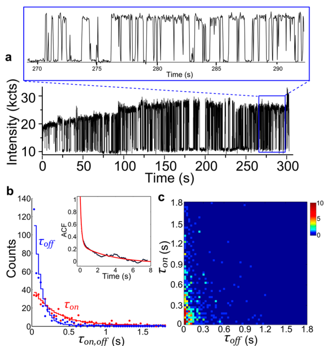
Figure 4. Single-molecule blinking dynamics of the zeolite H-ZSM-5 trapped 4-methoxystyrene-derived emitters in n -heptane. (a) Fluorescence intensity trajectory of a highly blinking molecule. (b) Histogram of lifetimes of the fluorescent (red dots) and dark states (blue dots) measured for the single-molecule trajectory shown in (a). Inset: autocorrelation function for the trajectory in (a). Red line is a biexponential fit, with exponential decay constants of t_1 = 0.16 \pm 0.02 s (fast-decay component) and t_2 = 3.6 \pm 0.8 s (slow-decay component). (c) Real 2-D frequency histogram of the (\tau_{on}, \tau_{off}) pairs as measured for the trajectory in (a). The color bar denotes the number of detected events for specific (\tau_{on}, \tau_{off}) values. The simulated 2-D histogram based on the experimentally measured (\tau_{on}, \tau_{off}) distributions in (b) is shown in SI Figure S4.
