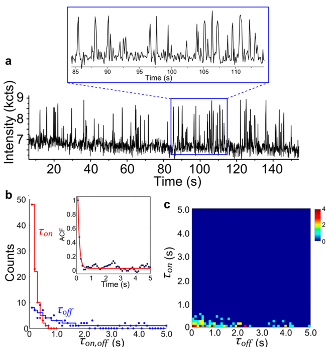
Figure 5. Single-molecule blinking dynamics of the zeolite H-ZSM-5 trapped 4-methoxystyrene-derived emitters in 1-butanol. (a) Fluorescence intensity trajectory of a highly blinking molecule. (b) Histogram of lifetimes of the fluorescent (red dots) and dark states (blue dots) measured for the single-molecule trajectory shown in (a). Inset: autocorrelation function for the trajectory in (a). Red line is a monoexponential fit, with exponential decay constant of t_1 = 0.11 \pm 0.02 s. (c) Real 2-D frequency histogram of the (\tau_{on}, \tau_{off}) pairs as measured for the trajectory in (a). The color bar denotes the number of detected events for specific (\tau_{on}, \tau_{off}) values. The simulated 2-D histogram based on the experimentally measured (\tau_{on}, \tau_{off}) distributions in (b) is shown in SI Figure S4.
