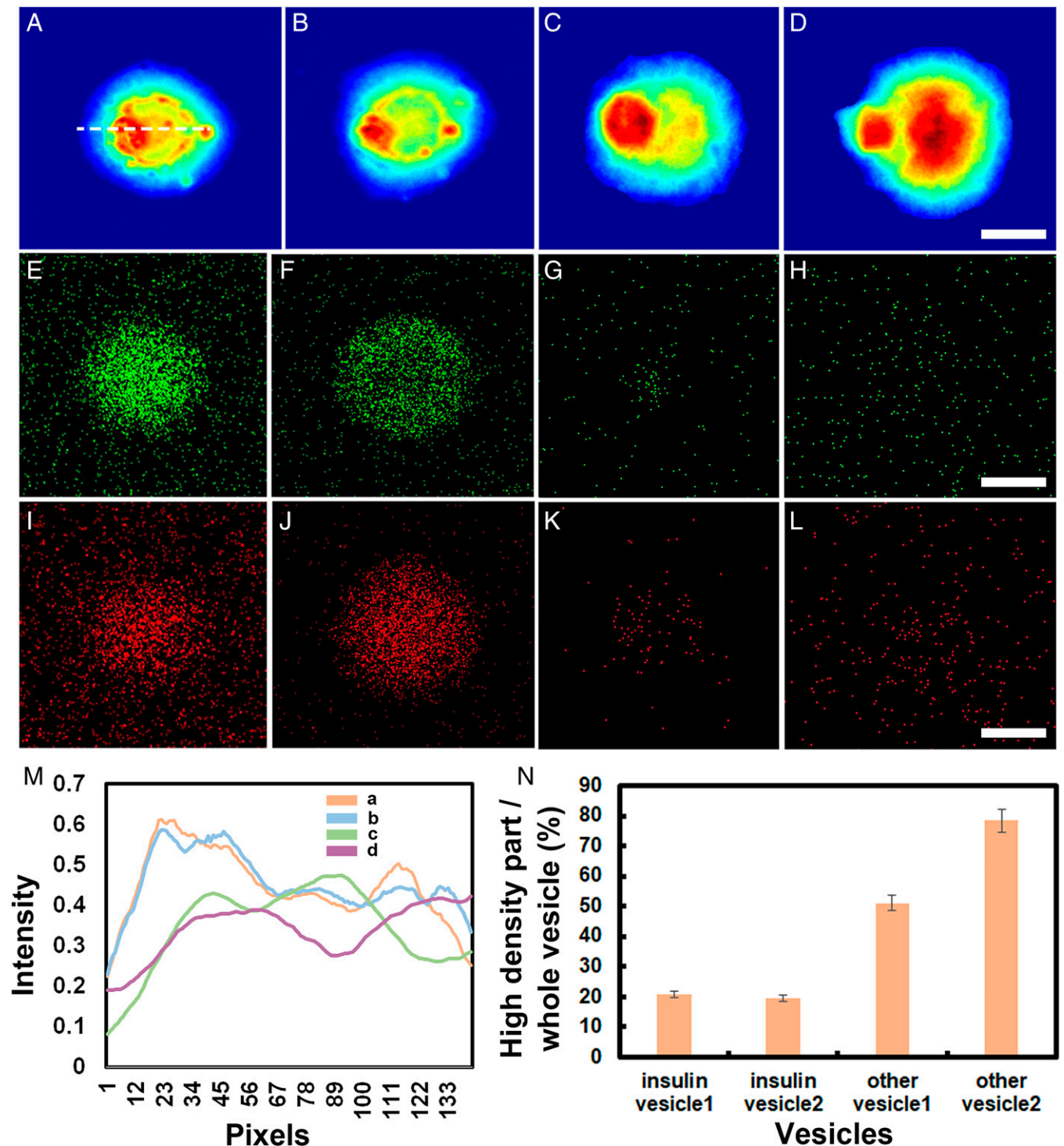
Fig. 5. Comparison of insulin vesicles and other vesicles. (A and B) Ptychography phase images of insulin vesicles. (C and D) Ptychography phase images of other types of vesicles. Scale bar, 200 nm. (E–H) EDS signals of Zn in the four vesicles A–D. Scale bar, 200 nm. (I–L) EDS signals of Ca in the four vesicles A–D. Scale bar, 200 nm. (M), Horizontal line scan (the white horizontal dashed line) across the center of the four vesicles. (N) The proportion of high-density area to the whole vesicle in the two types of vesicles. Percentage error.
