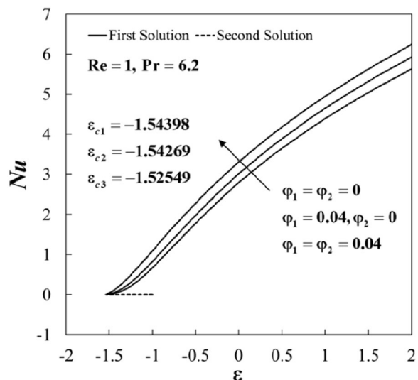
Figure 3. Plot of Nu against \varepsilon for different values of \varphi_1 and \varphi_2 .
