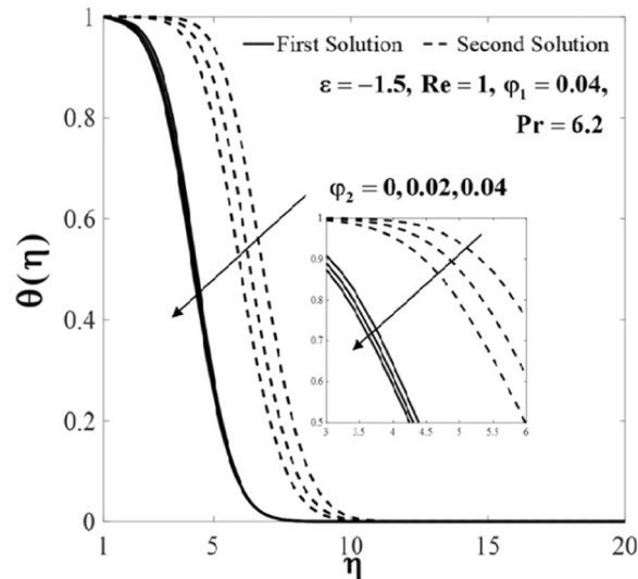
Figure 7. Plot of \theta(\eta)_f for different values of \varphi_2 .
