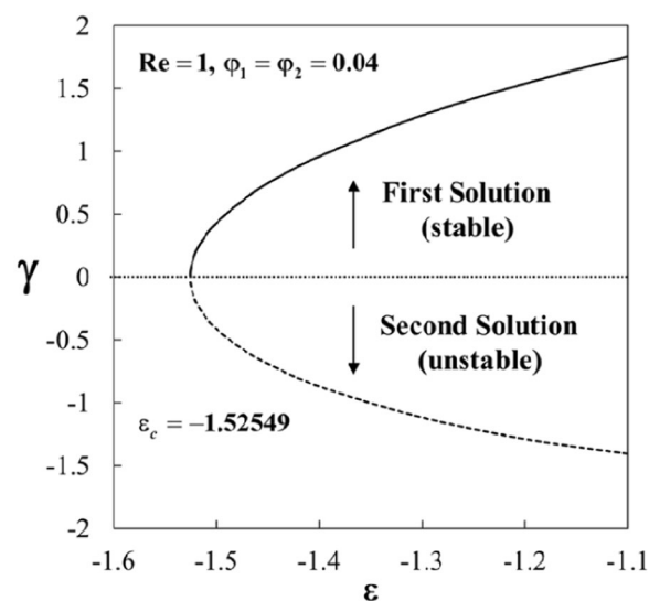
Figure 12. Plot of \gamma against \varepsilon for F''(1) = 1 .
