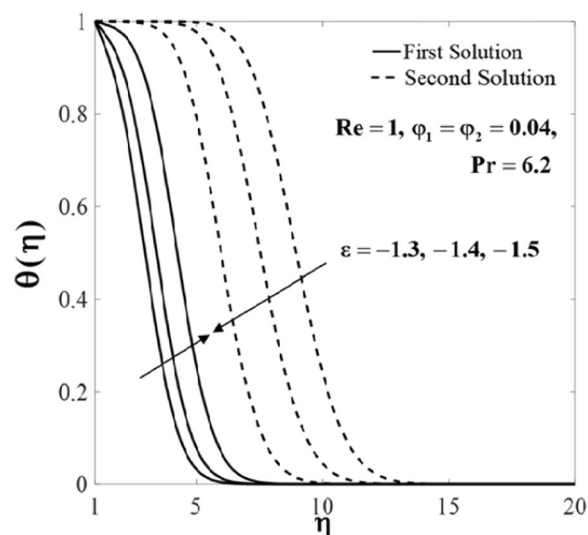
Figure 11. Plot of \theta(\eta) for different values of \varepsilon .
