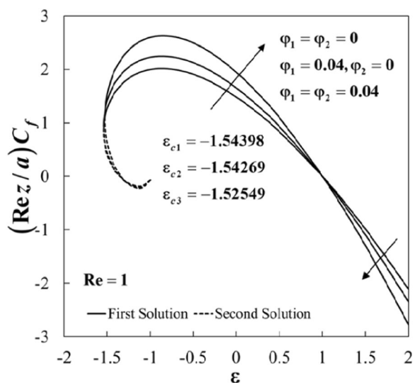
Figure 2. Plot of (Re z/a)C_f against \varepsilon for different values of \varphi_1 and \varphi_2 .
