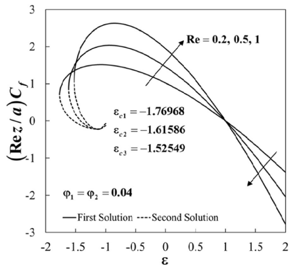
Figure 4. Plot of (Re z/a)C_f against \varepsilon for different values of Re .
