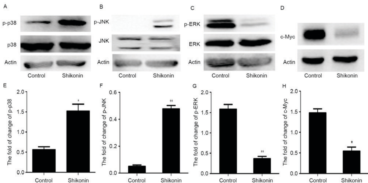
Figure 6. Effect of shikonin on the expression of mitogen-associated protein kinases and c-Myc. (A-D) NB4 cells were treated with 0.3 \mu\text{mol/l} shikonin for 24 h, and protein expression was measured by western blotting. (E-H) Quantification analysis of western blotting. * P < 0.05 , ** P < 0.01 vs. control. JNK, Jun N-terminal kinase; ERK, extracellular signal-regulated kinase.
