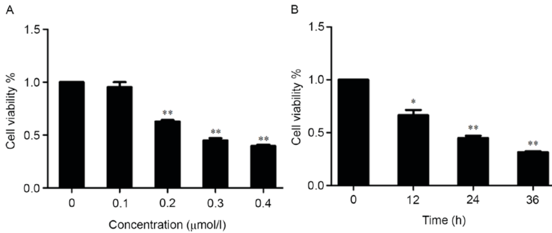
Figure 1. Treatment with shikonin inhibited human leukemia NB4 cell proliferation. (A) NB4 cells were treated with 0.1-0.4 μmol/l shikonin for 24 h. **P<0.01 vs. 0 μmol/l shikonin. (B) NB4 cells were treated with 0.3 μmol/l shikonin for 12, 24 and 36 h. CCK-8 results demonstrated that shikonin inhibited NB4 cells growth in dose and time-dependent manner. *P<0.05, **P<0.01 vs. time 0.
