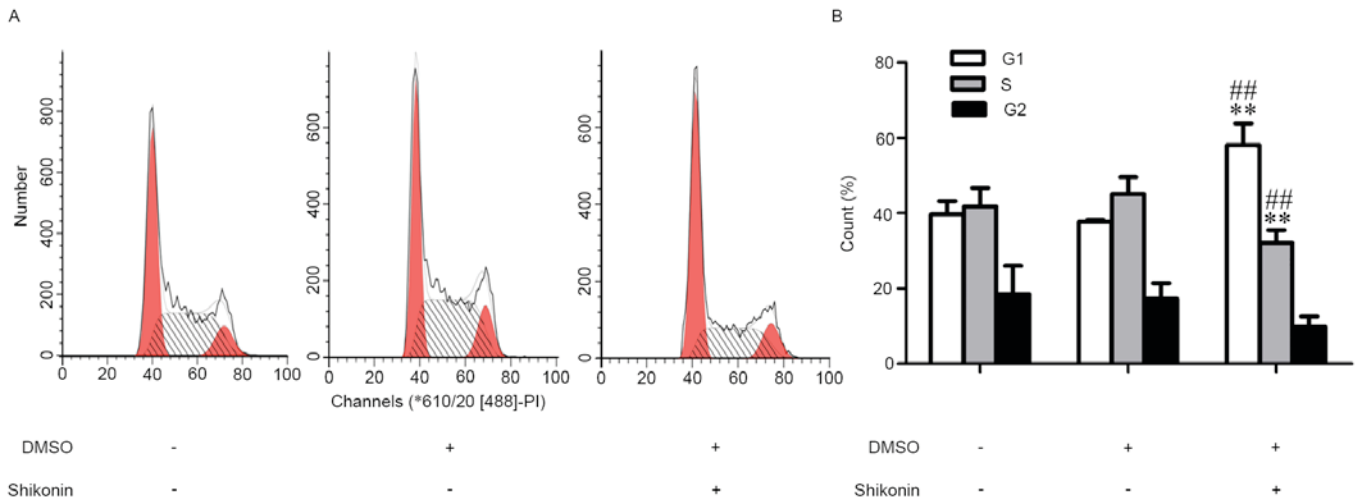
Figure 3. Changes in the cell cycle distribution in NB4 cells. (A) Treatment of 0.3 μmol/l shikonin in NB4 cells for 24 h induced the cell cycle arrest in the G1 phase. (B) Quantification of these data. ##P<0.01 vs. blank control; **P<0.01 vs. DMSO. DMSO, dimethylsulfoxide.
