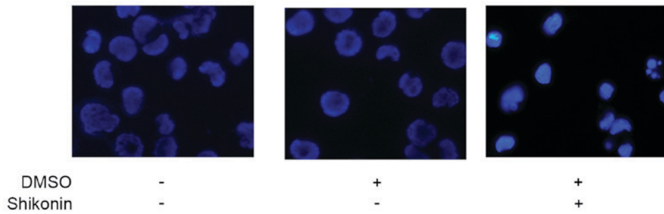
Figure 2. Effect of shikonin on nuclear morphology of NB4 cells was observed by fluorescence microscopy (magnification, x400). DMSO, dimethylsulfoxide.
