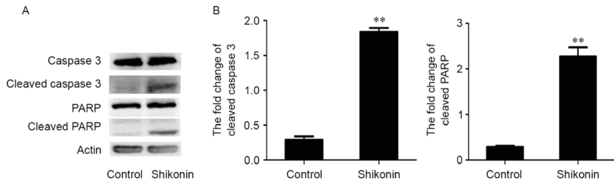
Figure 5. Effect of shikonin on the expression levels of apoptosis related proteins. (A) NB4 cells were treated with 0.3 \mu\text{mol/l} shikonin for 24 h. The expression levels of cleaved caspase-3 and cleaved PARP were increased. The expression levels of caspase-3 and PARP were not changed. (B) Quantification analysis of western blotting. ** P < 0.01 vs. control. PARP, poly ADP-ribose polymerase.
