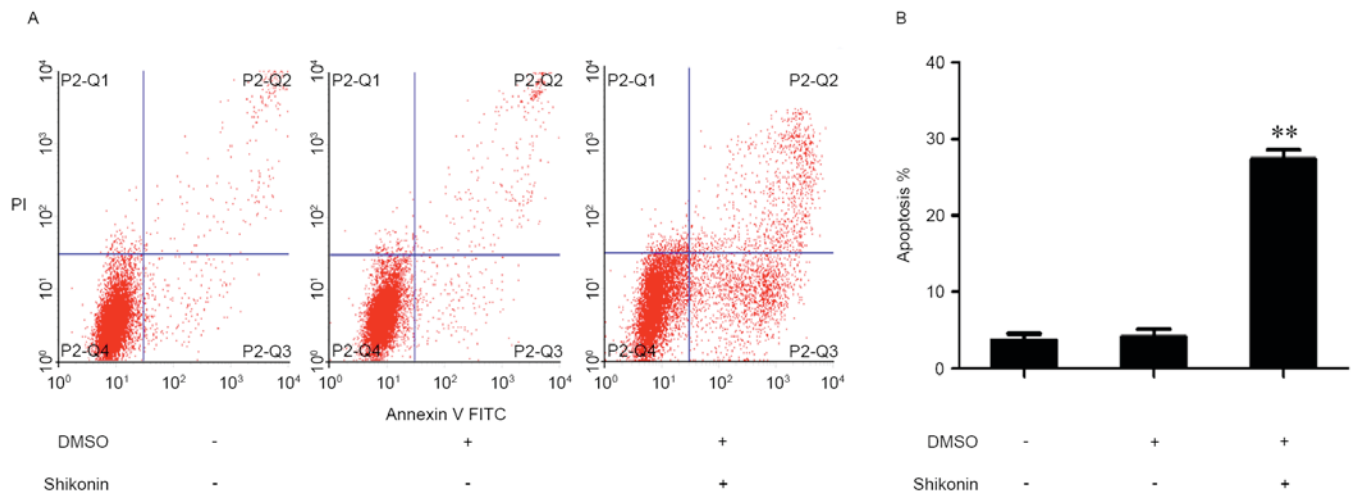
Figure 4. Shikonin increased NB4 cells apoptosis. (A) NB4 cells were treated with 0.3 \mu\text{mol/l} shikonin for 24 h, then cell apoptosis was detected by flow cytometry. The percentage of apoptosis cells was increased by shikonin treatment. (B) Quantification of these data. ** P < 0.01 vs. control. DMSO, dimethylsulfoxide; FITC, fluorescein isothiocyanate.
