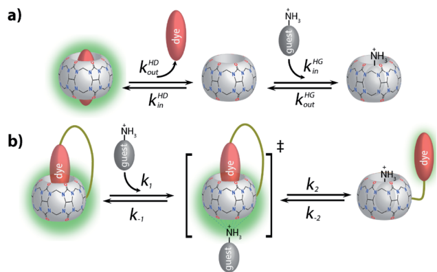
Fig. 9 (a) Schematic representation of a S_{N1} -type-mechanism for the guest-exchange process on analyte-induced conformational changes of non-covalent CB7 \supset dye reporter pair complexes; (b) schematic representation of a S_{N2} -type-mechanism for the guest-exchange process on analyte-induced conformational changes of CB7 -dye conjugates.
