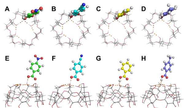
Fig. 2 Hypothetical conformations of (A and E) [\alpha\text{-CD} + p\text{NBA-H}]^- , (B and F) [\alpha\text{-CD} + p\text{CBA-H}]^- , (C and G) [\alpha\text{-CD} + \text{BA-H}]^- and (D and H) [\alpha\text{-CD} + p\text{MBA-H}]^- . (A to D) Top views and (E to H) side views.
