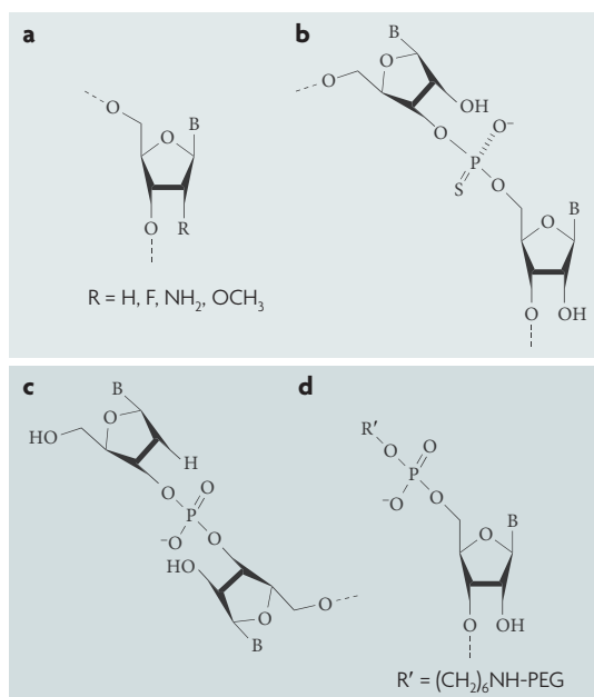
Figure 1 | Aptamer modifications. a | Nucleotides can be modified by replacing the 2' position with either a fluoro (F), amino- (NH 2 ) or O -methyl (OCH 3 ) group for enhanced nuclease resistance. These modified nucleotides can be introduced either chemically or enzymatically. b | Bridging phosphorothioates can be incorporated enzymatically. c | End caps that involve reversing the polarity of the chain can be incorporated during chemical synthesis. d | Linkers are often inserted at the 5'-ends of aptamers by either chemical or enzymatic means to provide handles for conjugation or to alter pharmacokinetic properties. B, base; PEG, polyethylene glycol.
