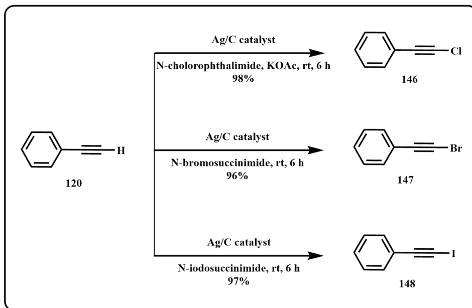
Scheme 44 Alkyne halogenation catalyzed by Ag/C catalytic system (Liu et al. 186 ).
