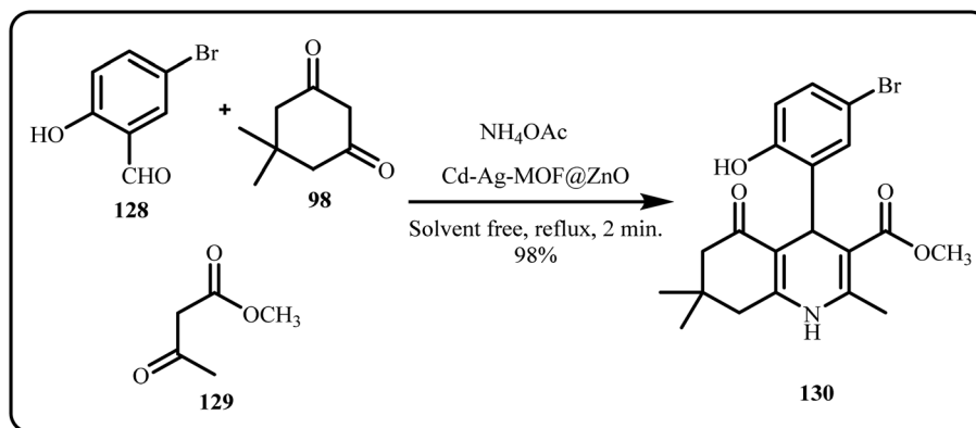
Scheme 38 Catalytic synthesis of polyhydroquinoline heterocycle derivatives using Cd-Ag-MOF@ZnO (Hoot et al. 175 ).
