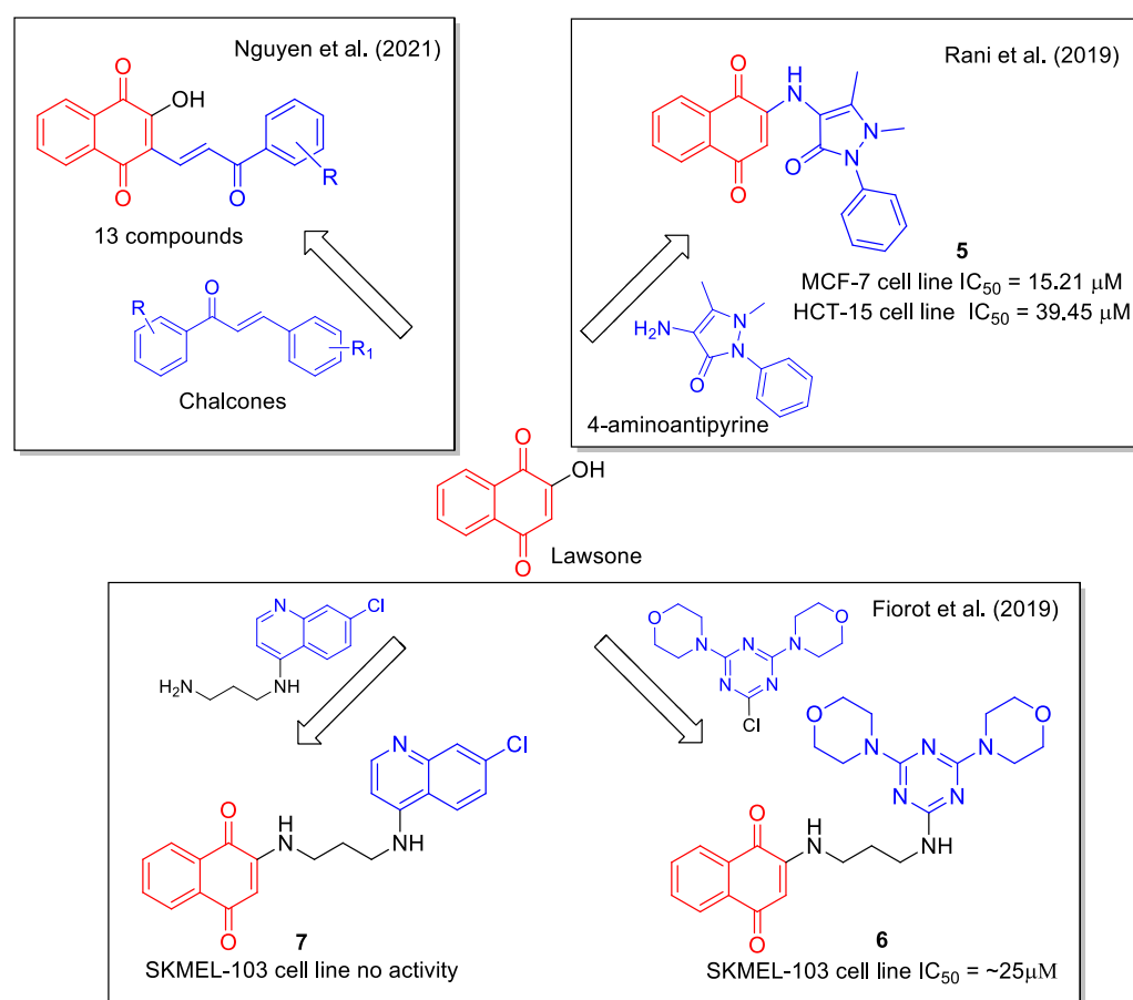
Figure 4. 1,4-Napthoquinone hybrids with aminoantipyridine as reported by Rani et al. [29], with chloroquinoline by Fiorot et al. [30] and with chalcone by Nguyen et al. [31].
