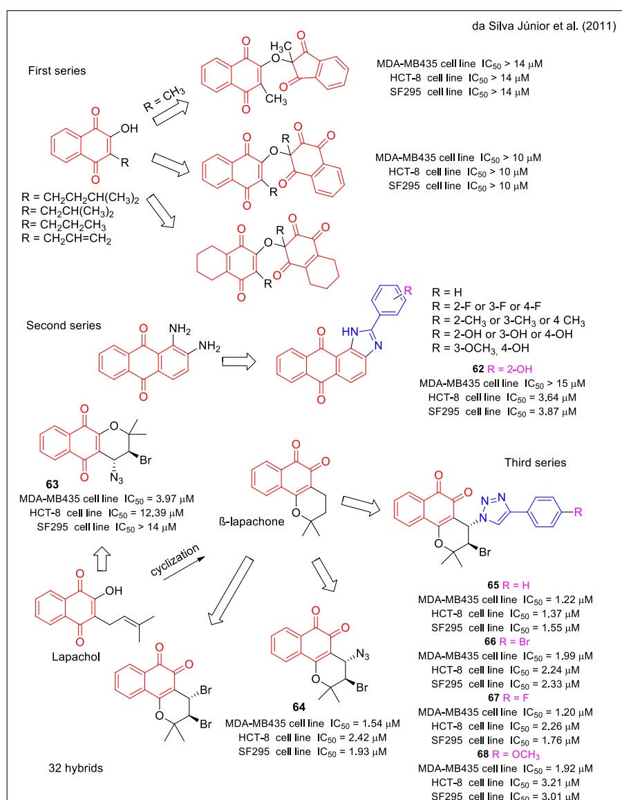
Figure 24. 1,4- and 1,2-Napthoquinone hybrids as reported by da Silva Júnior et al. [66].
