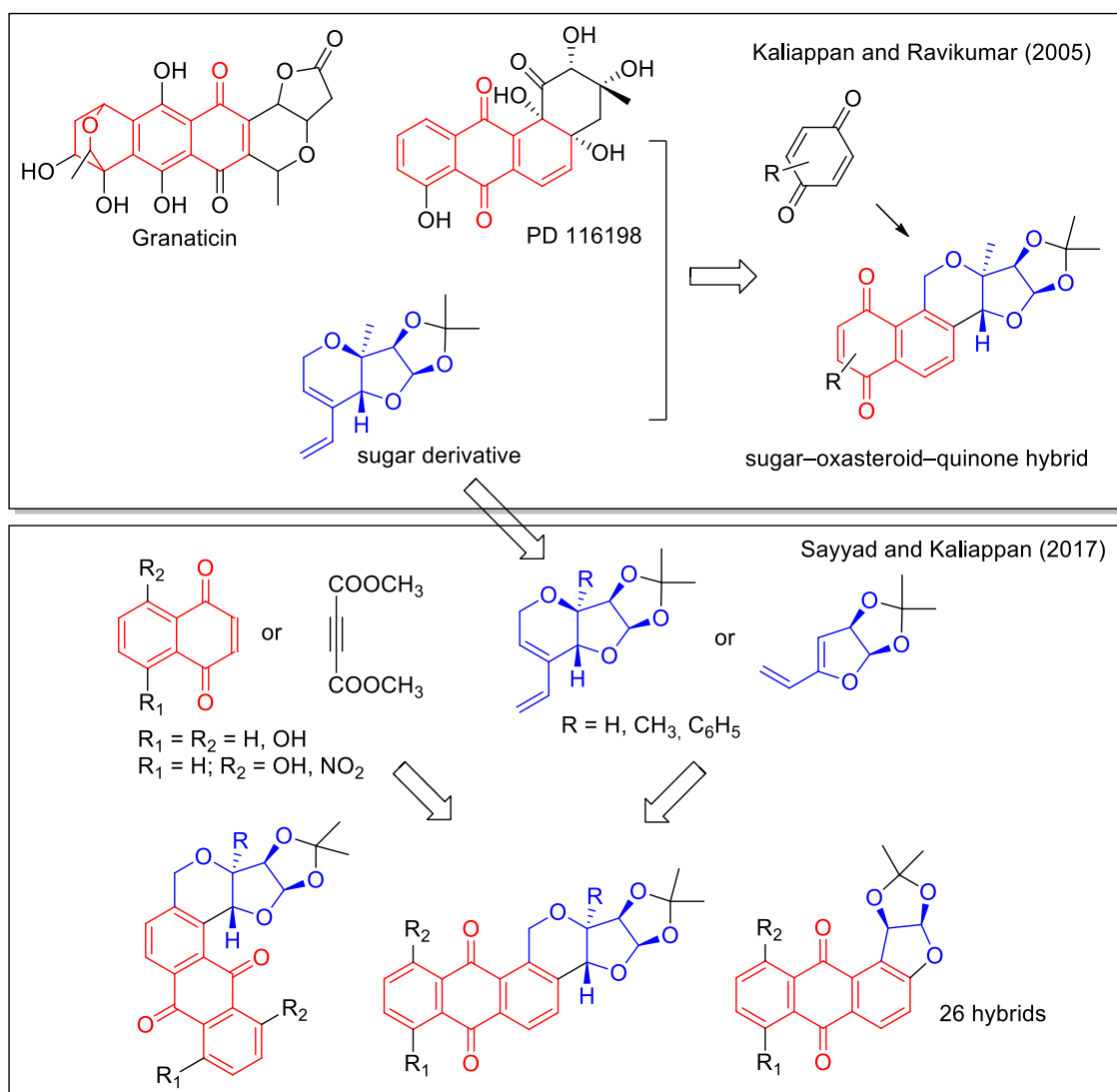
Figure 16. Sugar-oxasteroid-quinone hybrids as reported as reported by Kaliappan and coworkers [49,50].
