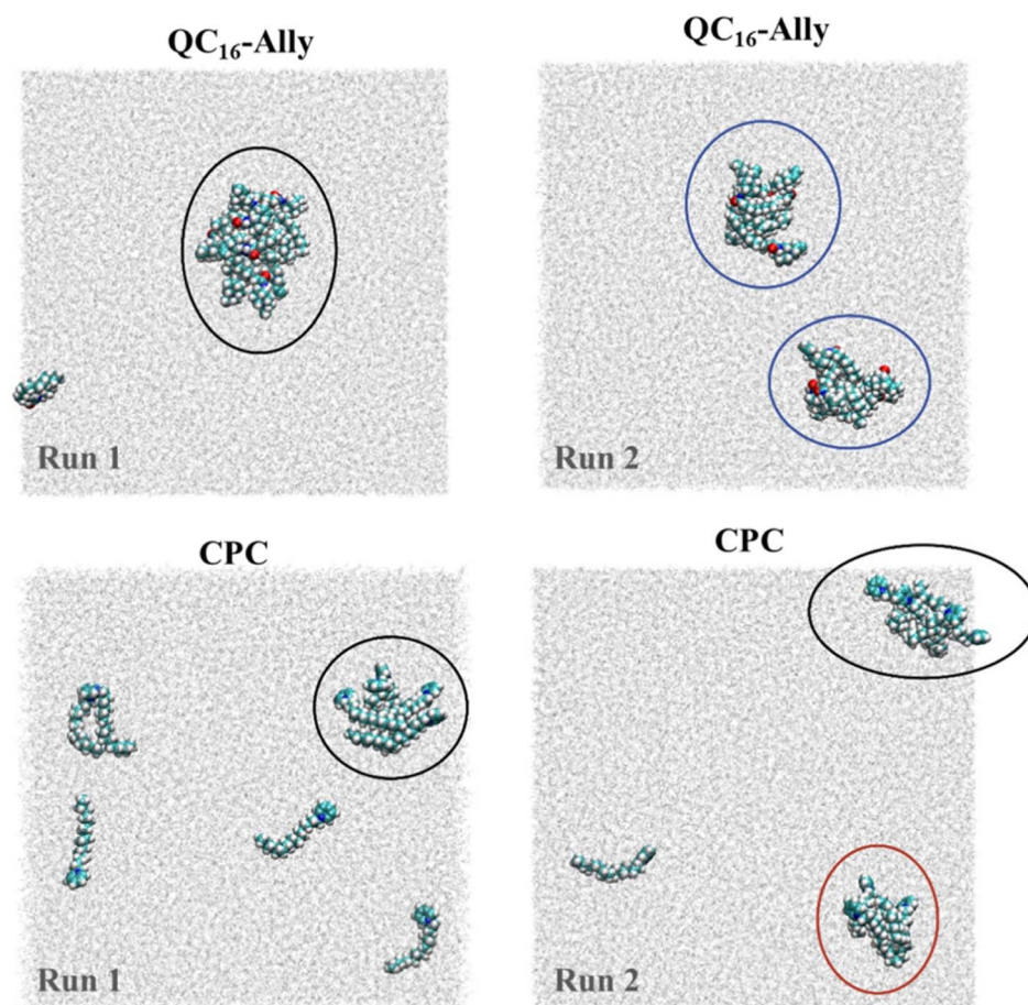
Fig. 6 Clusters/aggregates formed at t = 100 ns, for QC 16 -Ally/water (top panel) and cetylpyridinium chloride/water, CPC/water (bottom panel) systems. Results of the two propagations shown (left and right columns), with the third simulation of each system omitted. Observed clusters/aggregates are denoted with ellipses (black – dominant cluster/aggregate, blue – two equally sized clusters/aggregates, red – smaller cluster/aggregate).
