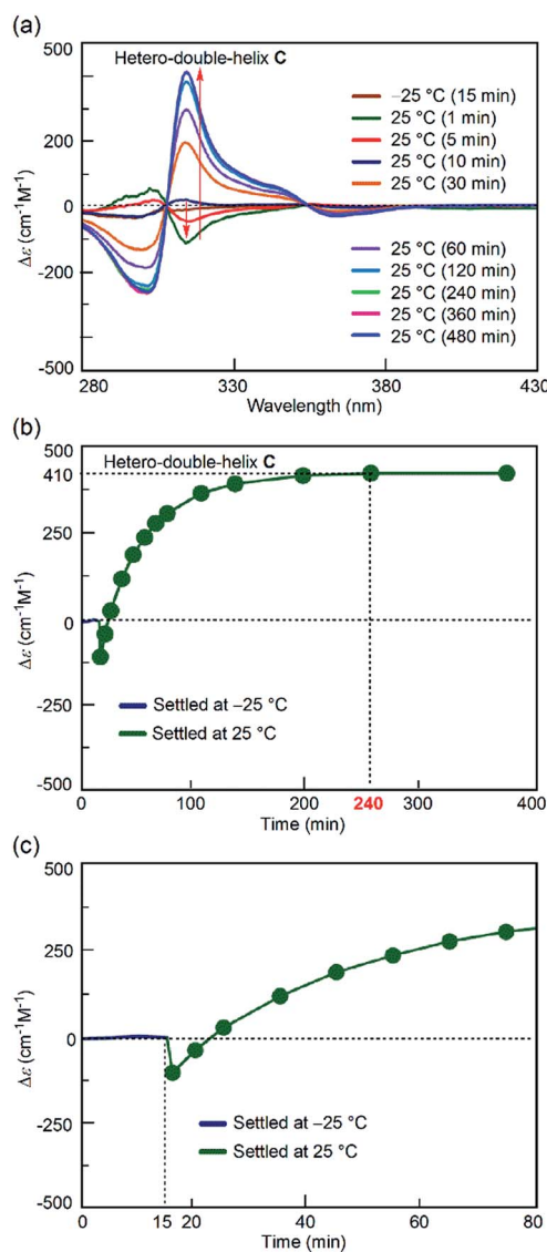
Fig. 3 (a) CD spectra and (b) \Delta\epsilon (315 nm)/time profiles of 1 : 1 ( P )-1/( M )-2 mixtures in fluorobenzene (total concentration, 5.0 \times 10^{-4} M) showing structural changes from the random coil A at 70 °C to the hetero-double helix C at 25 °C under the freezing–defrosting/rapid heating conditions. (c) A magnification of (b).
