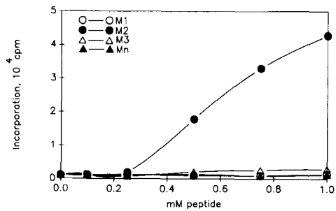
Figure 3. Stimulation of microtubule assembly with synthetic peptides. Varying concentrations of each peptide were added to 1.6 mg/ml tubulin and 0.4 mg/ml microtubule protein in the presence of [ ^3\text{H} ]GTP and a GTP-regenerating system (MacNeal et al., 1977). After reaching steady state, the amount of GTP incorporation was determined by the filtration assay of Maccioni and Seeds (1978) as modified by Wilson et al. (1982) (see Materials and Methods).
