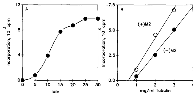
Figure 4. Assembly curve and critical concentration plot of peptide-induced assembly. Phosphocellulose-purified tubulin (1.0 mg/ml) was incubated with m_2 peptide (1.0 mM) at 37°C. At the indicated times in A, the amount of GTP incorporation was determined as described earlier. In B, varying concentrations of tubulin plus microtubule seeds, prepared as described in Materials and Methods, were mixed with or without m_2 peptide (1.0 mM) at 37°C and assayed for GTP incorporation 30 min after addition of microtubule seeds.
