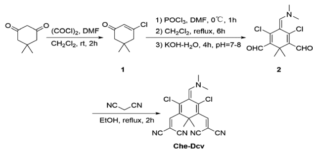
Scheme 1 Synthetic route of Che-Dcv .
