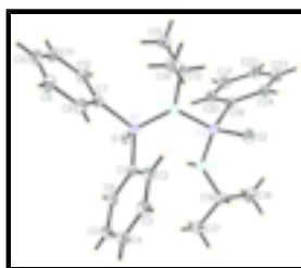
Fig. 1. The molecular structure of the title compound showing the labelling scheme. Atomic displacement ellipsoids are drawn at the 30% probability level.
