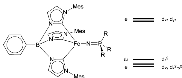
Figure 4. Chemical structure of the \text{Fe}^{\text{II}} complexes with \text{R} = \text{H, Me, } ^n\text{Pr, Ph} . Schematic diagram of the d-orbital splitting corresponding to \text{C}_{3v} point group symmetry.
