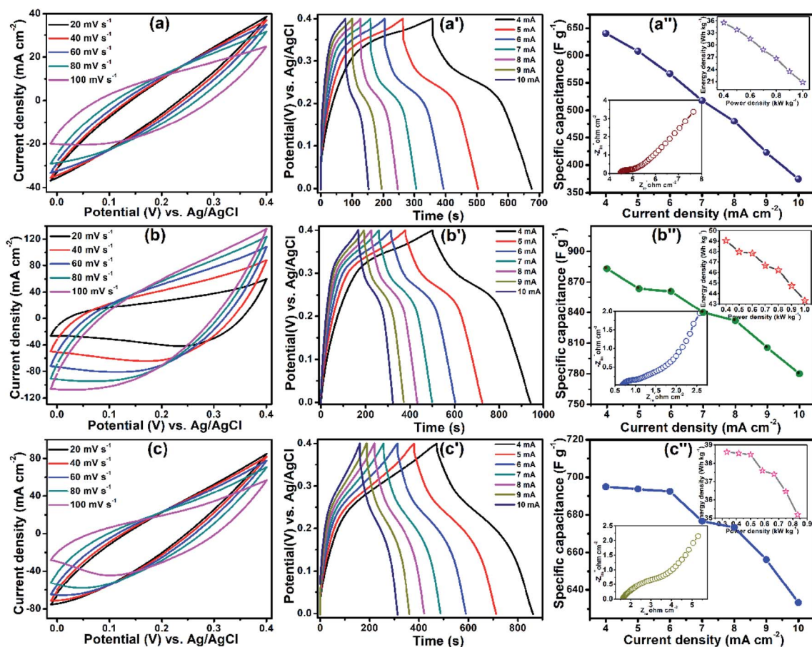
Fig. 6 CV curves of (a) NZ-0.5, (b) NZ-1, and (c) NZ-2 at different scan rates and the corresponding GCD curves (a'–c') and graphs of specific capacitance (a''–c'') measured at different current densities. Insets are the corresponding Nyquist plots and Ragone plots, respectively, measured at various current densities.
