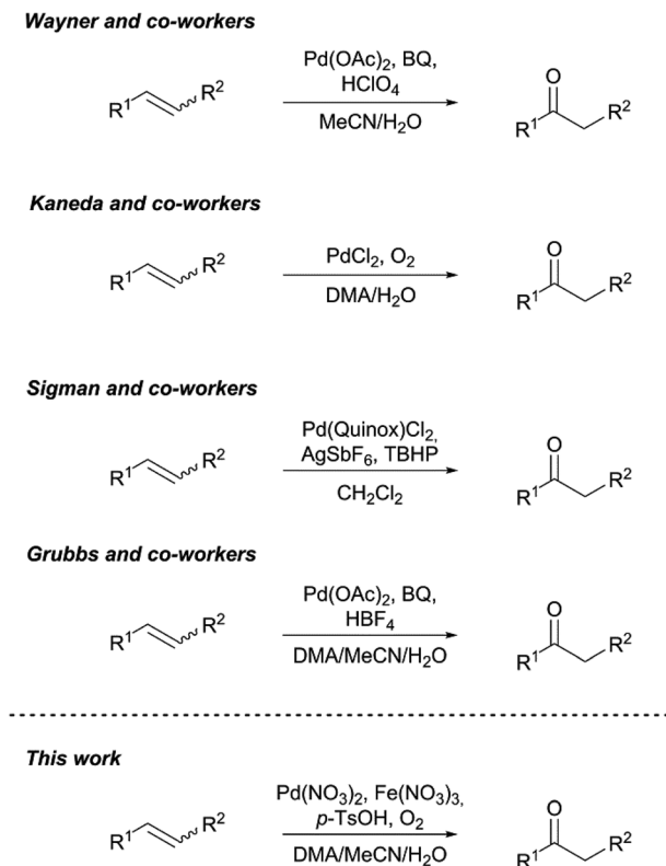
Scheme 1 Reported Wacker type oxidation reactions of cyclic and internal olefins.
