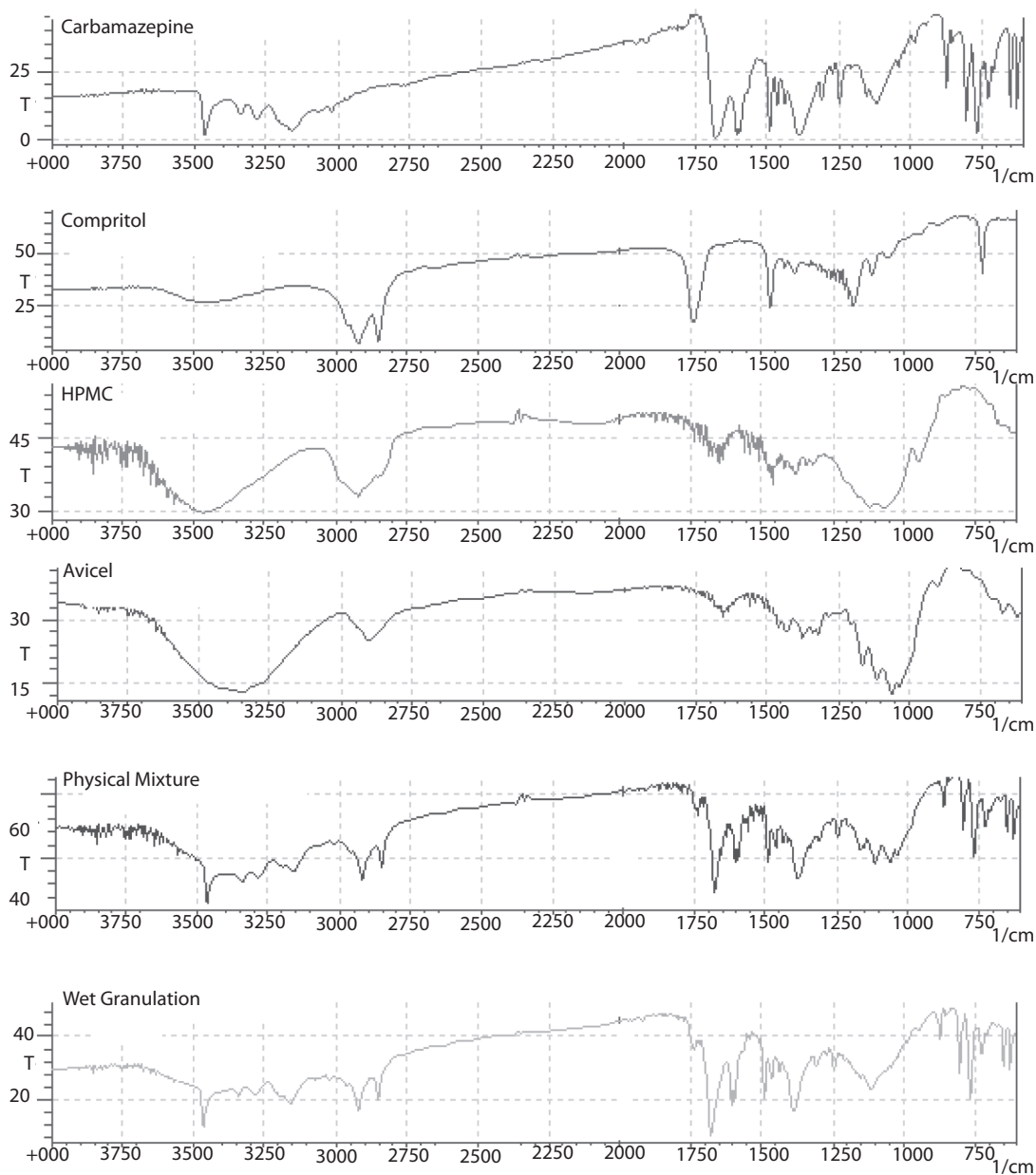
Figure 2. Infrared spectra of pure CBZ, Compritol ® , HPMC, and Avicel ® and of physical and granulated mixture at 7:2:1 Compritol ® :HPMC:Avicel ® weight ratio.
