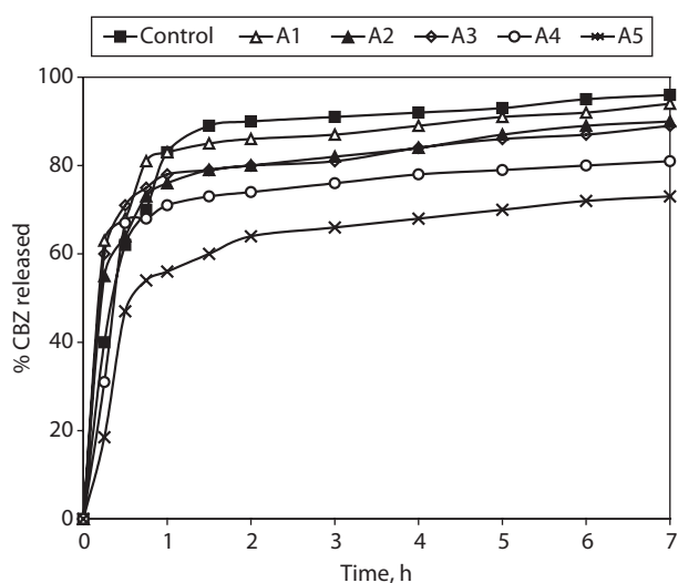
Figure 3. % Carbamazepine released from Compritol:HPMC matrix granules (size fraction 710–500 \mu\text{m} ).
