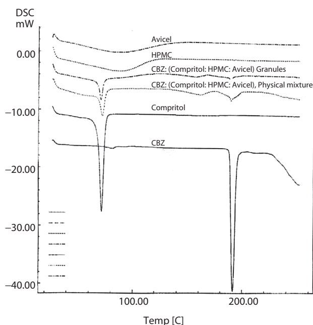
Figure 1. DSC thermograms of pure CBZ, Compritol®, HPMC, and Avicel® and of physical and granulated mixture at 7:2:1 Compritol®:HPMC:Avicel® weight ratio.
