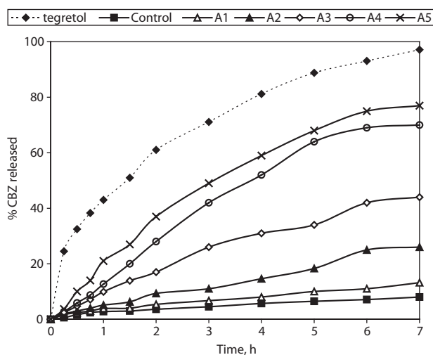
Figure 4. % Carbamazepine released from prepared matrix tablets and commercial product Tegretol®.
