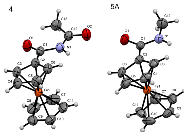
Figure 2. Molecular structures of 4 and 5A. Thermal ellipsoids are drawn for the probability of 50 % and hydrogen atoms are depicted as spheres of arbitrary radii.
