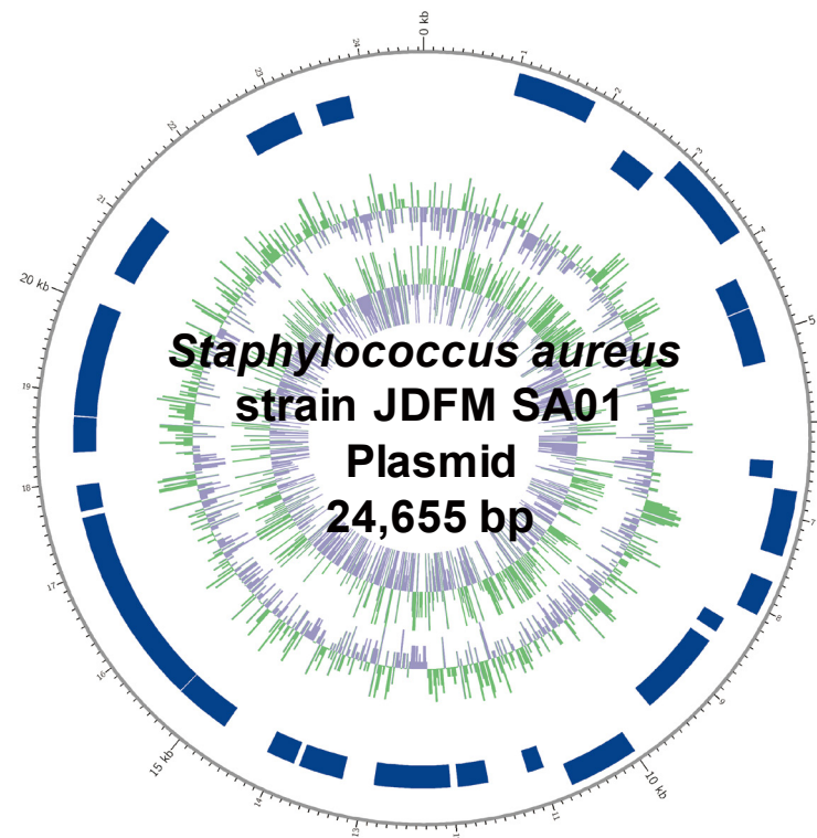
Fig. 1. Circular chromosome and plasmid maps of Staphylococcus aureus strain JDFM SA01. Marked characteristics are shown from outside to the center; coding DNA sequences (CDSs) on forward strand, CDS on reverse strand, tRNA, rRNA, GC content and GC skew. (A) Chromosome, (B) Plasmid.
