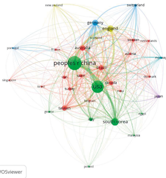
FIGURE 7: Network map of countries with at least 20 publications.
