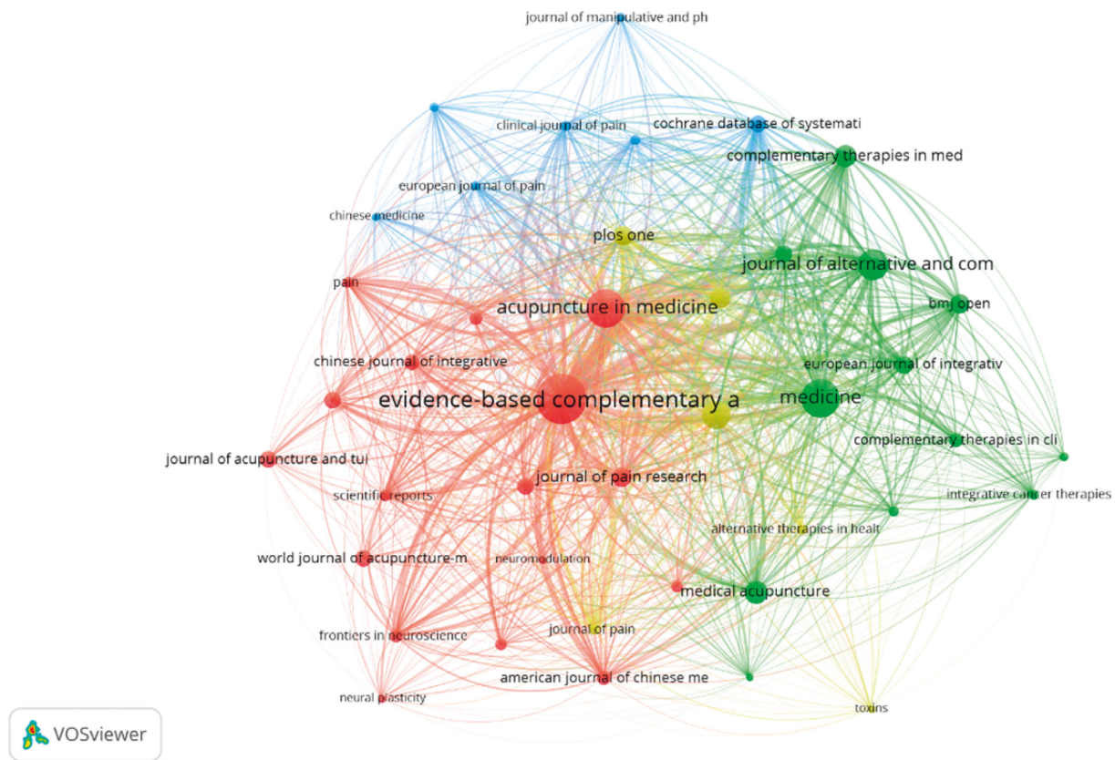
FIGURE 4: Bibliometric coupling of journals.
