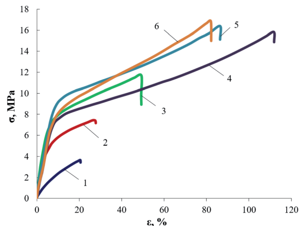
Fig. 2 Tensile tests for AEPA–PU, obtained at ratios of [\text{PIC}] : [\text{AEPA}] = 1 (1), 1.1 (2), 1.2 (3), 1.3 (4), 1.4 (4), 1.5 (6), wt%.
