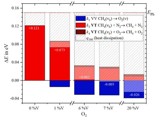
Fig. 5. Representation of the contributions of individual collision reactions to the photoacoustic signal amplitude for selected N_2:O_2 matrix compositions as a bar chart. The red dashed horizontal line indicates the energy of a light quantum in eV. The overlaid white diagonally hatched area illustrates the absolute heat dissipation q_{100} .
