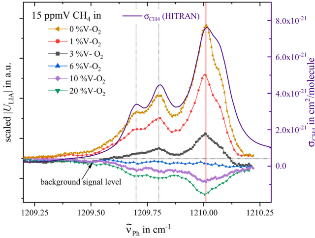
Fig. 2. Amplitude modulated photoacoustic spectra of 15 ppmV methane in pure \text{N}_2 (yellow) and successively substituting \text{N}_2 by \text{O}_2 (red to green). The purple line depicts the absorption cross-section from HITRAN database.
