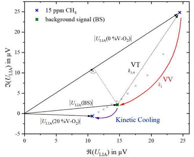
Fig. 3. The photoacoustic measurement signals for 15 ppmV \text{CH}_4 at 13 different \text{N}_2/\text{O}_2 ratios is presented as a complex vector diagram (blue crosses). The measurement points at the minimum (pure \text{N}_2 ) and maximum (20%V \text{O}_2 ) concentrations are highlighted in bold, while the background signals are shown as a green point cloud. The colored curved arrows illustrate relaxation processes and do not represent vectors.
