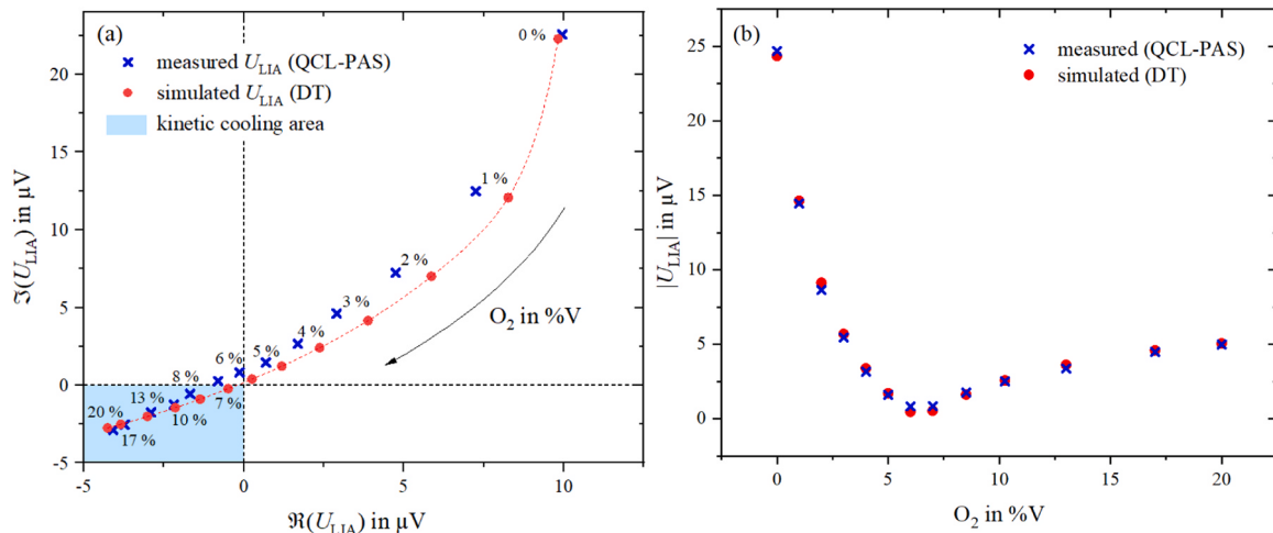
Fig. 4. Measured PA signals from Fig. 3 after offset-correction (blue crosses) and DT-simulated signals (red dots) are presented in a complex vector diagram (a) and their absolute values plotted as a function of O_2 concentration (b).
