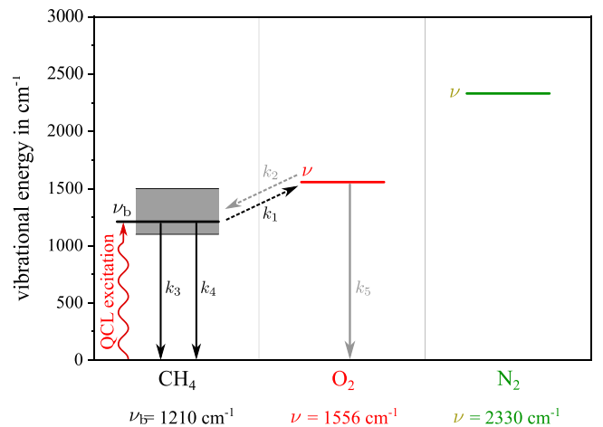
Fig. 1. Simplified Jablonski diagram of a two-level system to predict the relaxation cascade of photoacoustic signal generation for methane monitoring in air. The grey shaded area highlights the dyad of \text{CH}_4 vibrations \nu_{\text{b}} [28].
