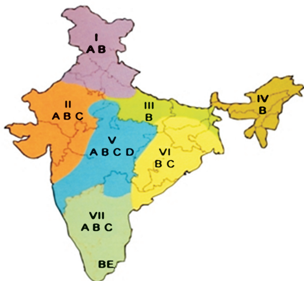
Fig. 3. Map of India showing geographical distribution of An. culicifacies complex (sibling species A, B, C, D, and E), and stratification (Divisions I-VII) for vector control options. (Source : Ref. 57).
