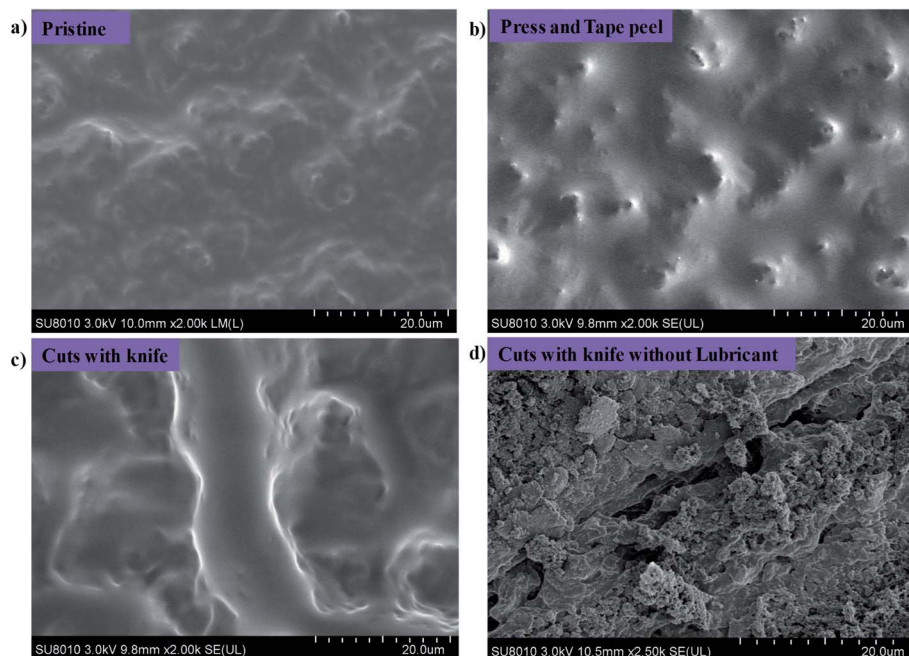
Fig. 16 (a–c) SEM images shows the mechanical stability of the candle soot slippery surface after subsection to pressing, tape peel, touching, and knife cuts. (d) SEM image of candle soot surface after applying cut without lubricant.
