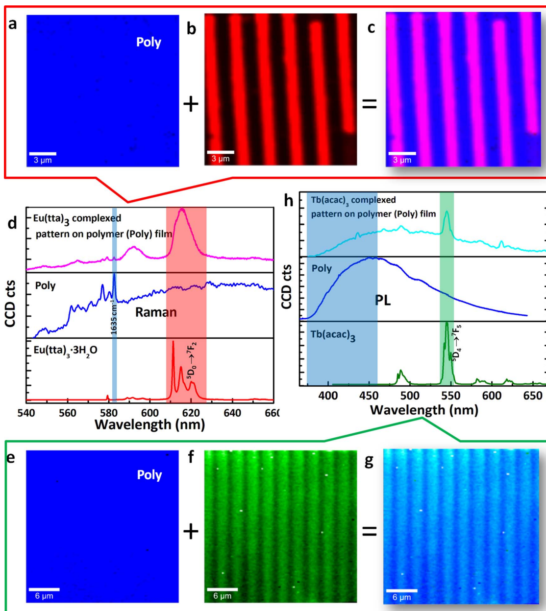
Figure 5 | Patterning of Eu(III) and Tb(III) inks coordinatively on a polymer surface. Raman/PL images of Eu(tta) 3 printed stripes on the polymer surface: (a), False color Image of 1635 cm -1 Raman peak corresponding to blue PL of polymer. (b), False color Image of the red PL peak (610–620 nm) from stripes. (c), Combined image of (a) and (b). (d), Spectra of Eu(tta) 3 complexed pattern on polymer surface, polymer and Eu(tta) 3 ·3H 2 O, the marker peaks are shown in violet and magenta color for polymer and Eu(tta) 3 , respectively. PL images of the Tb(acac) 3 pattern on polymer surface: (e), False color Image of a peak in the region between 376–472 nm corresponding to blue PL of polymer. (f), False color Image of the green PL peak in the region between 540–550 nm from stripes shown in green color. (g), Combined image of (e) and (f). (h), Spectra of Tb(acac) 3 complexed pattern on polymer surface, polymer and Tb(acac) 3 ·H 2 O, the marker peaks are shown in violet and green color for polymer and Tb(acac) 3 ·H 2 O, respectively.
