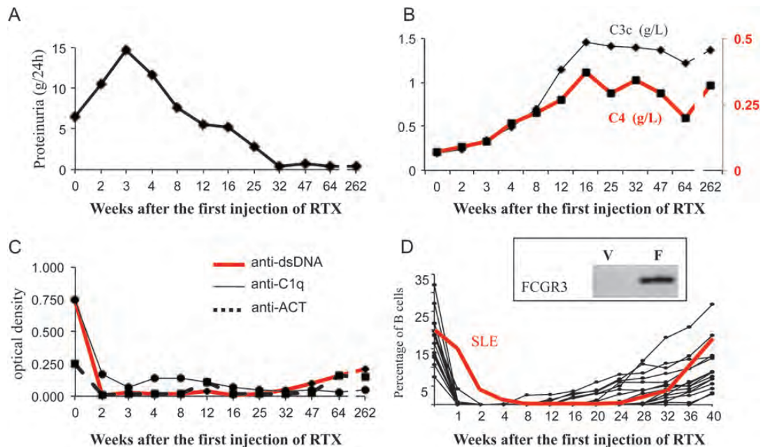
Fig. 1. Longitudinal variations of (A) proteinuria; (B) C3c and C4 complement fractions; (C) anti-dsDNA Ab, anti-C1q Ab and anti-alpha actinin (ACT) Ab and (D) percentage of peripheral blood B cells in a lupus nephritis patient re-treated with RTX and compared with 14 primary Sjögren's syndrome patients treated with RTX. The 14 SS patients displayed the three FCGR3A genotypes (5 were F/F, 9 were V/F and 1V/V). Of particular note, the SS patient who achieved B-cell depletion at 2 weeks was FCGR3A 158F/F. In the figure, allele-specific PCR is showing an FCGR3A 158F/F genotype.
