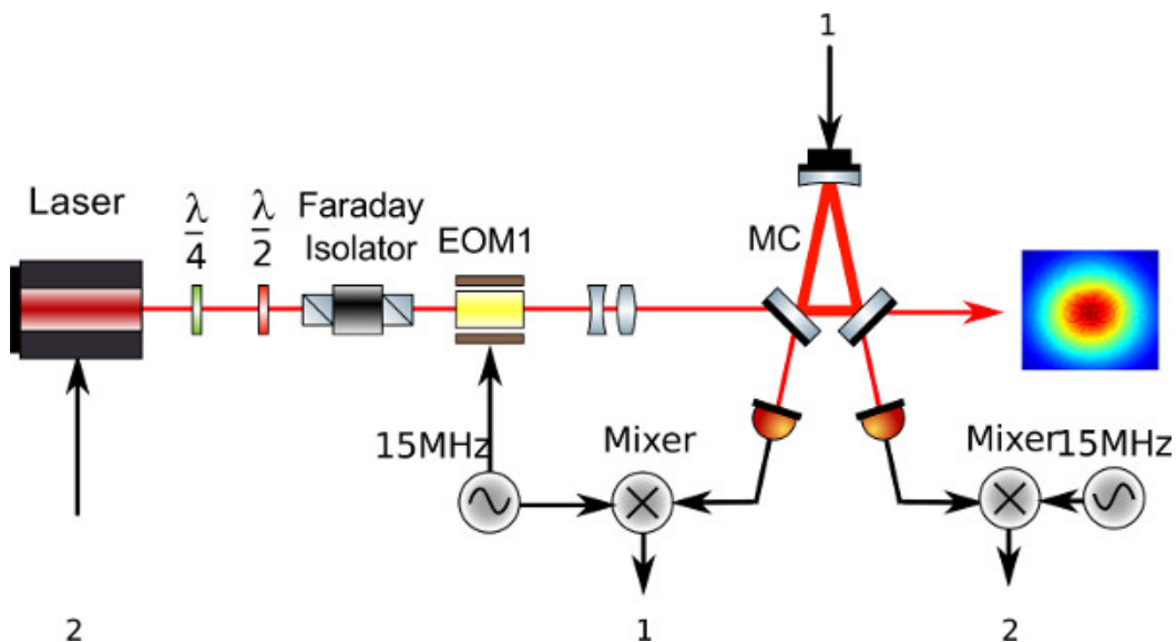
Figure 3. Sketch of a conventional setup for production and stabilization of HG_{00} beams.
