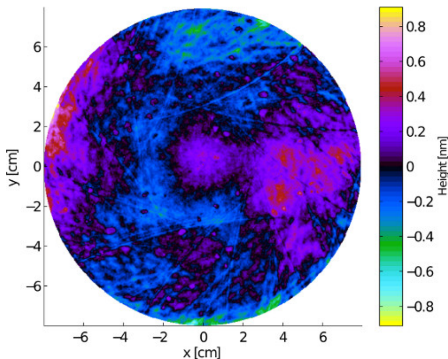
Figure 11. An example of a mirror surface map for one of the Advanced LIGO optical mirrors 19 .
