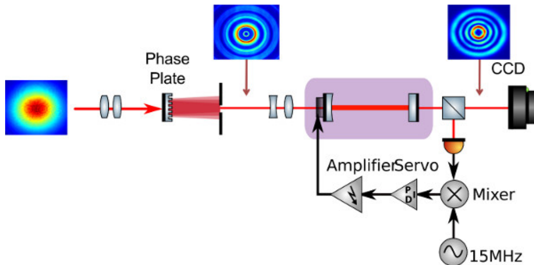
Figure 4. A sketch of the experimental setup discussed in this paper. The HG_{00} beam is first mode-matched to a desired waist size via a telescope then injected on the phase plate. The main diffracted beam is separated from the higher diffraction orders with an aperture and then sent to the Mode Cleaner cavity. A photodiode is used to extract the error signal for controlling the cavity length. The beam intensity is analyzed by a CCD camera.
