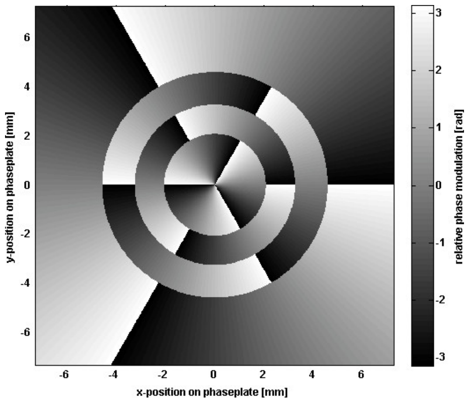
Figure 5. Phase modulation profile to convert a HG_{00} mode to LG_{33} mode.
