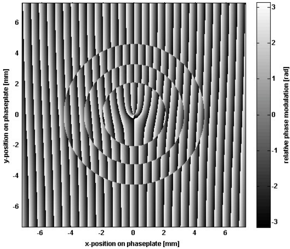
Figure 6. Example of blazed phase modulation profiles for generating LG_{33} modes.
