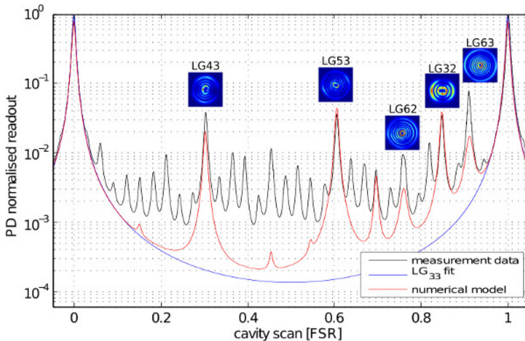
Figure 10. Light power transmitted by a linear cavity as a function of the cavity length, when injecting a beam generated by the phase plate. The resonant peaks at 0 and 1 FSR correspond to the desired LG_{33} mode. A fit to this dominant mode is shown for comparison (blue line). The red curve shows the result of the numerical model, based on the modal content described in Table 2 . Pictures of the unwanted beams to be filtered by the cavity are shown in the insets.
