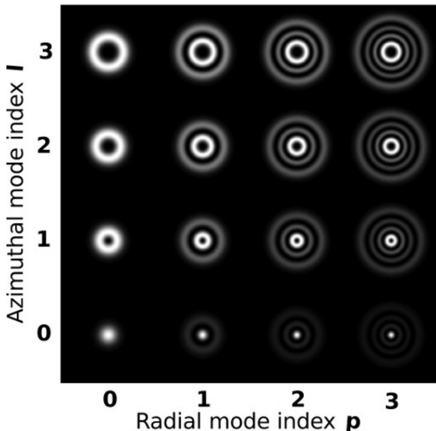
Figure 2. Intensity patterns for helical LG modes up to order 9. The intensity patterns are normalized to have the same peak intensity, for visibility.
