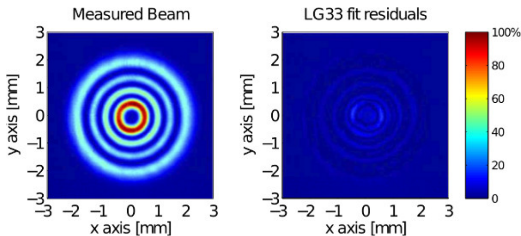
Figure 12. Intensity profile of a 82.8 W LG 33 beam transmitted by a linear cavity (left) compared with fit residuals (right).
