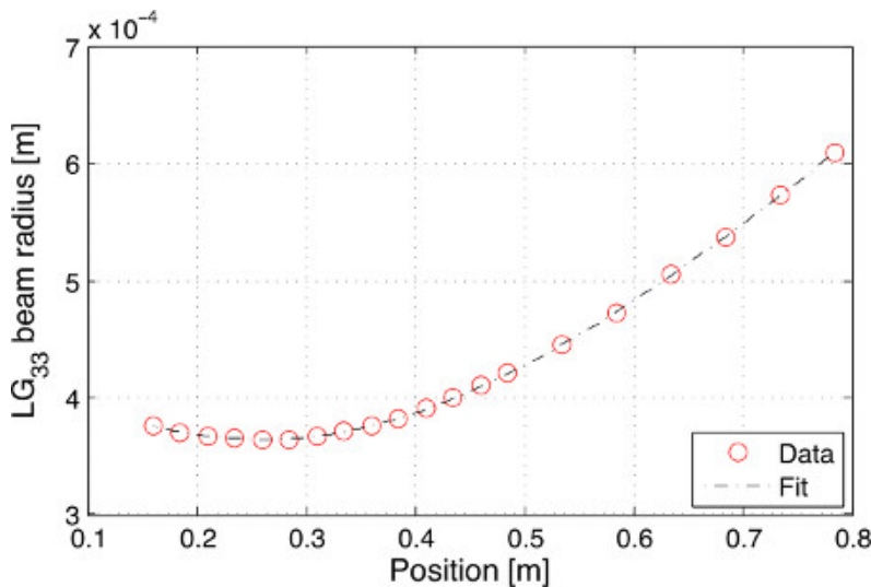
Figure 9. Profile of an LG_{33} beam with Gaussian fit shown for comparison.
