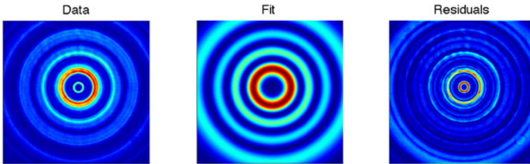
Figure 8. Example of beam intensity profile fitting applied to a real LG_{33} beam transmitted from a phase plate (left) compared to fit results (center) and residuals of fit (right). Click here to view larger figure.
